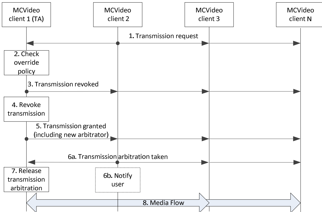
Figure 7.7.2.8-1: Transmission override
