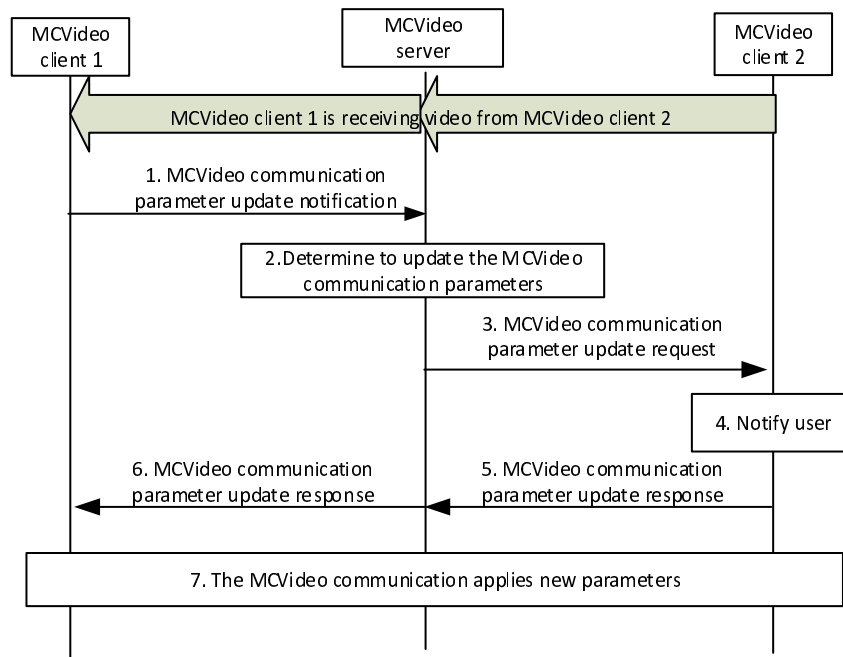
Figure 7.17.3.4-1: Receiving user triggered MCVide adaptation in private communication
