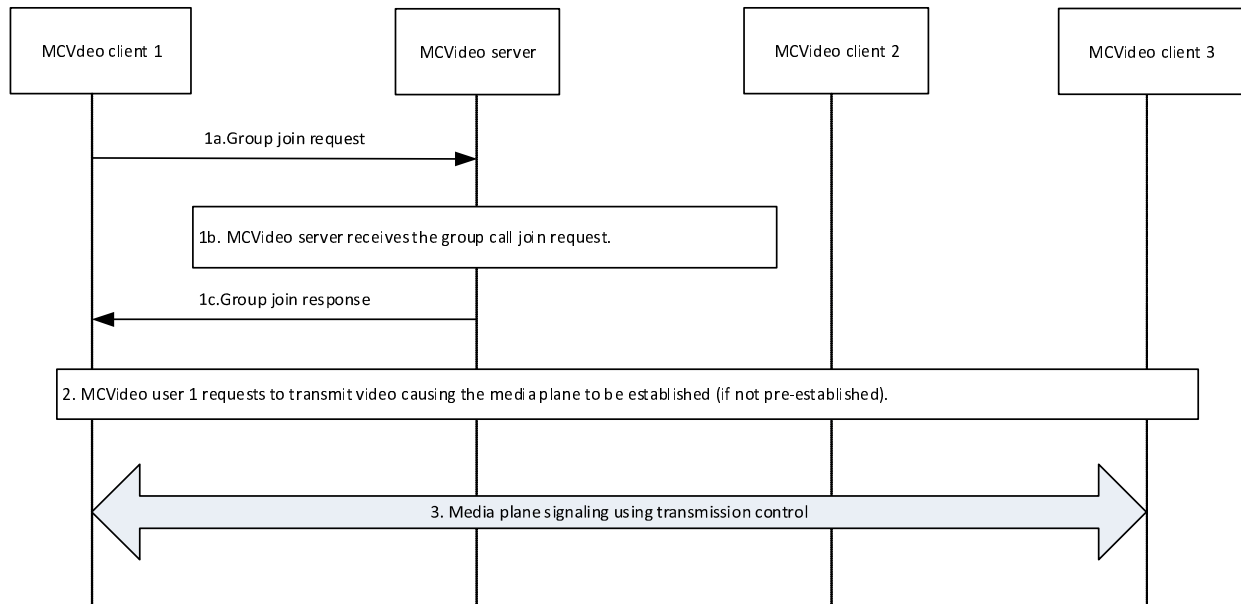
Figure 7.1.2.3.1.2.2-1: MCVideo chat group call
