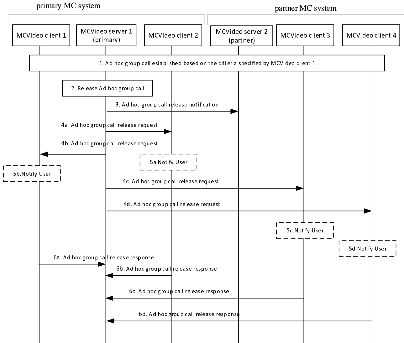
Figure 7.19.3.2.3-1: MCViideo server releases an ad hoc group call and stops the determination of ad hoc group call participants involving multiple MCViideo systems
