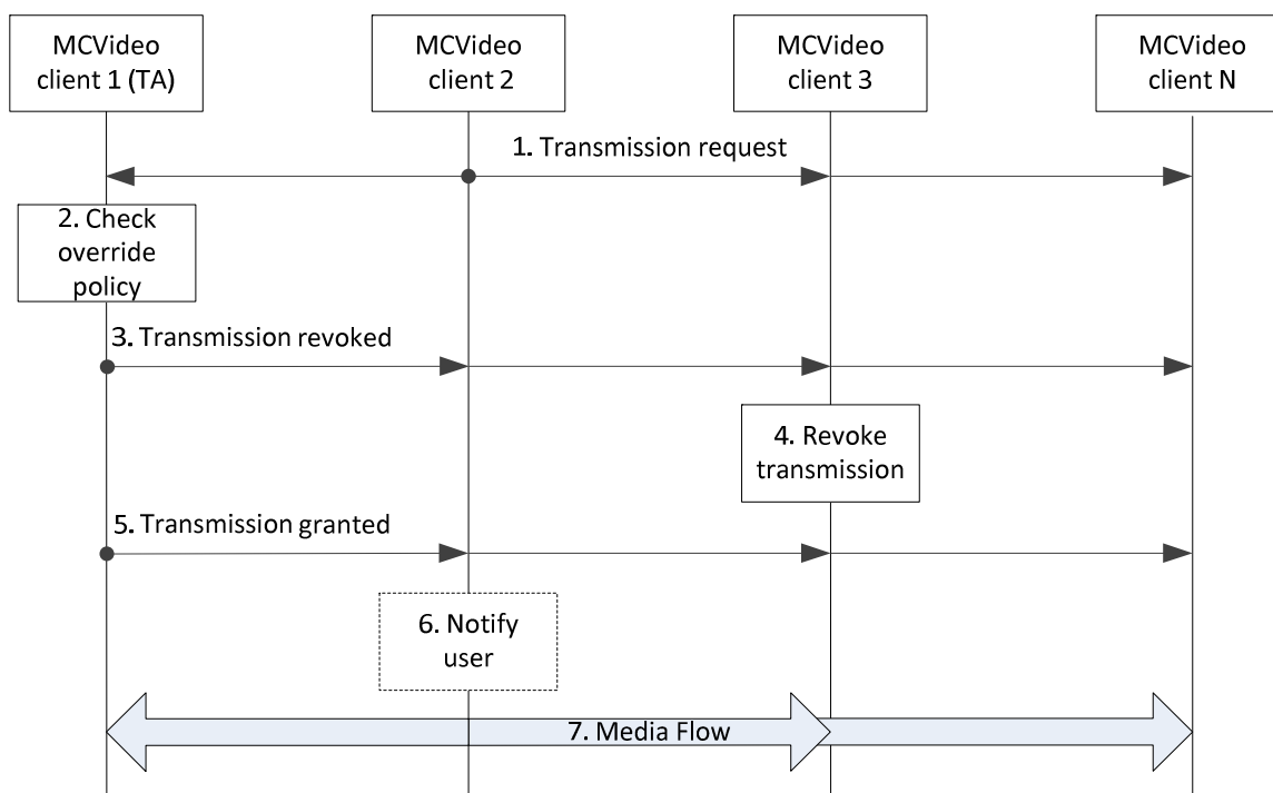
Figure 7.7.2.7-1: Transmission override
