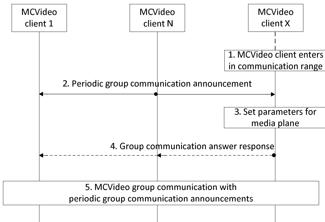
Figure 7.1.3.4.2-1: Passive join to MCVideo group communication
