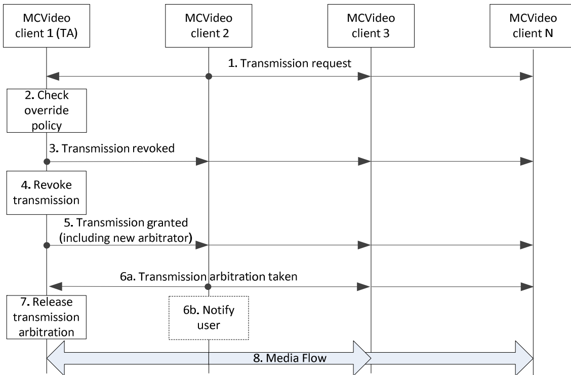
Figure 7.7.2.8-1: Transmission override
