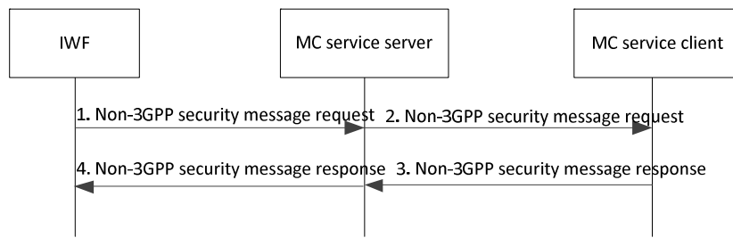
Figure 10.12.2.3-1: Non-3GPP security, from the IWF to MC service client
