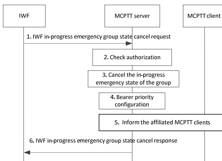
Figure 10.6.2.3.1-1: LMR user initiated in-progress emergency group state cancel of an interworking group defined in the MCPTT system
