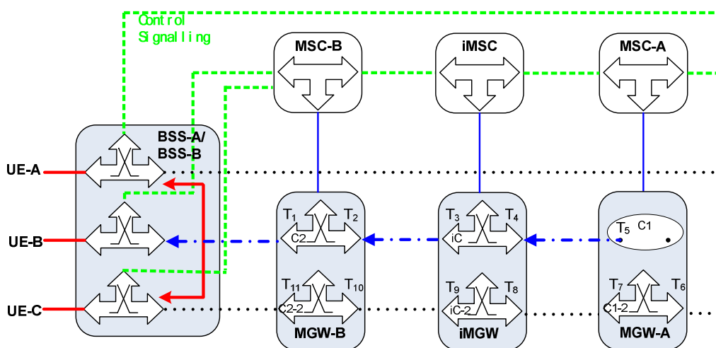
Figure 13.5.2.2.1.1: Connection Model for Accept Incoming call, original call is held
