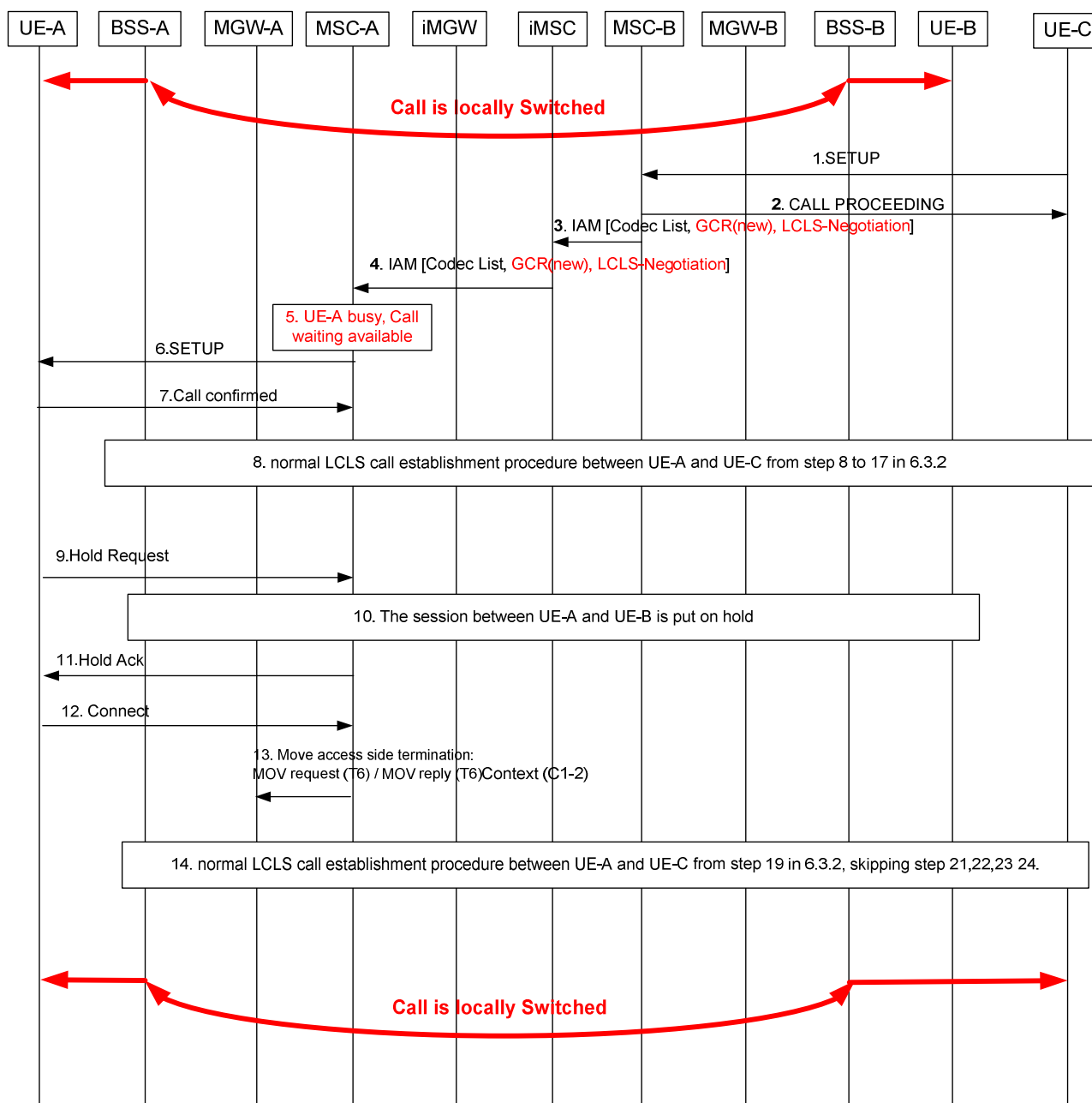
Figure 13.5.2.2.1: Accept Incoming call, original call is held
