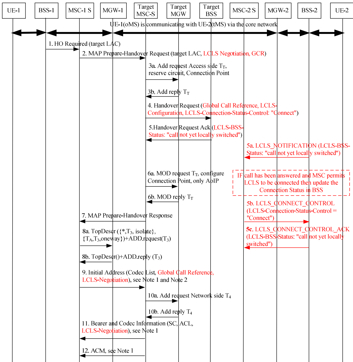
Figure 8.4.2.2.4.2.1: Initial phase of Inter-MSC Handover establishing Local Switching
