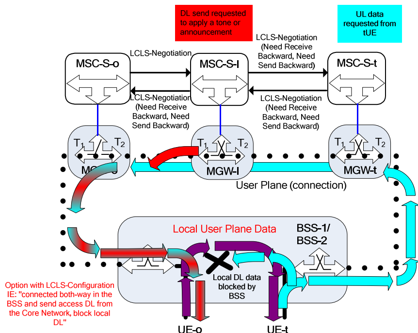
Figure A.1.5: iMSC requesting UL data from tUE plus sending DL data to oUE
