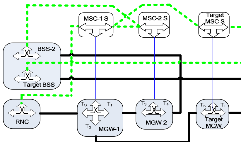
Connection Model 2: During Handover, T_2 is isolated from T_5 , T_1 is one-way connected to T_2
