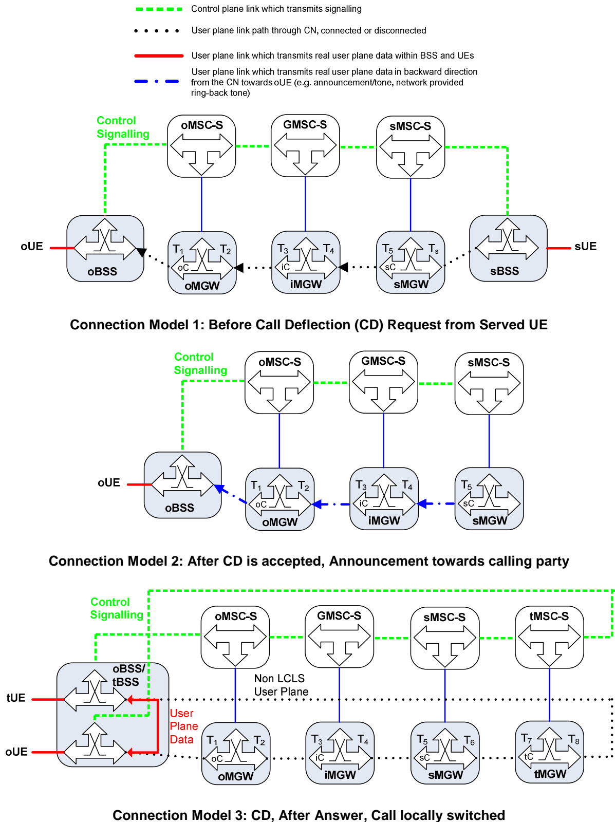
Figure 13.2.6.1.1: Connection Model for Call Deflection
