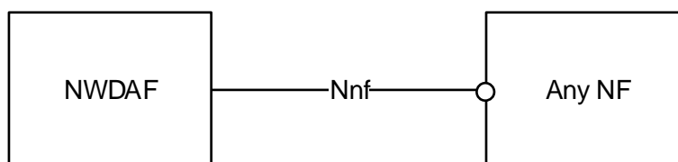
Figure 4.2-1: Data Collection architecture from any 5GC NF
