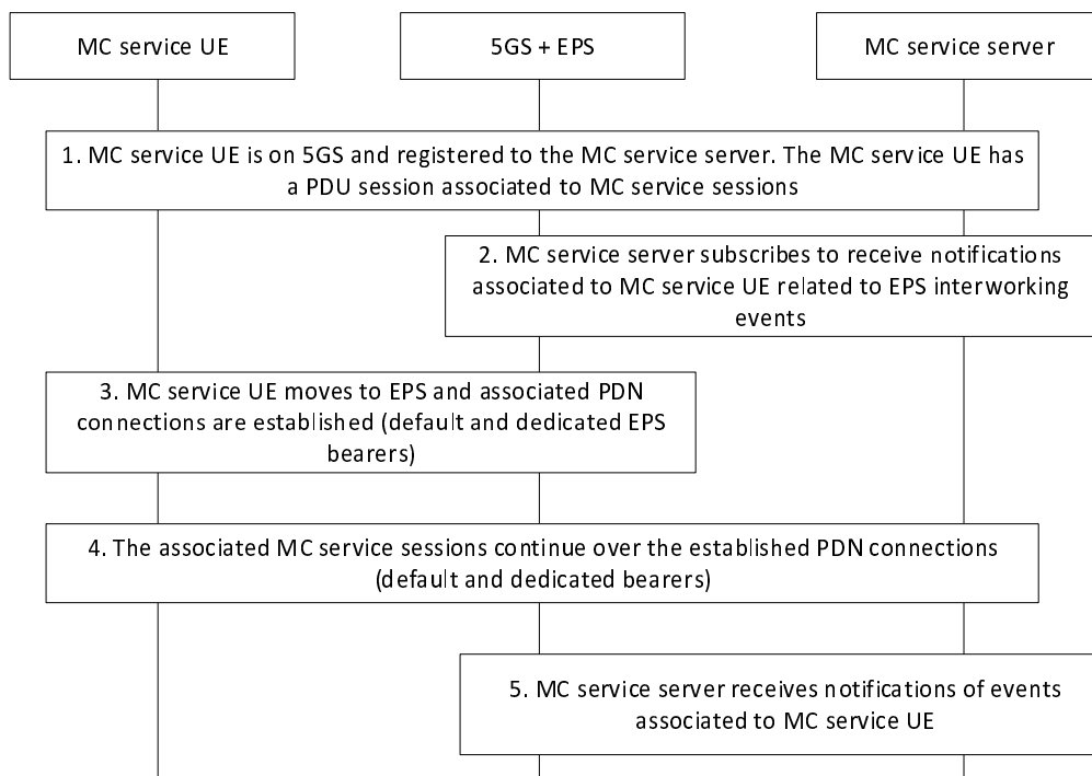
Figure 7.4.3-1: Network notifications of EPS interworking related events
