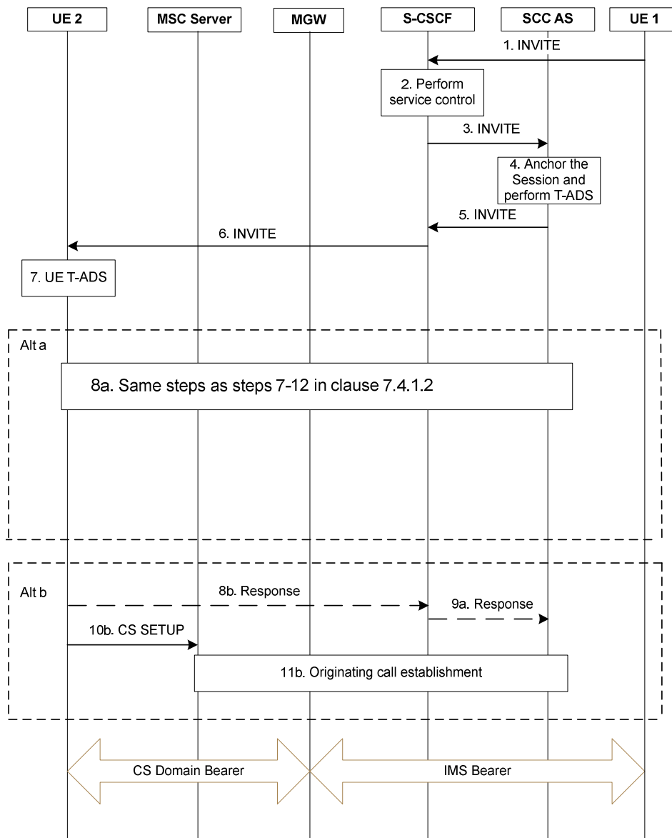
Figure 7.4.1.3-1: Fallback using UE T-ADS
