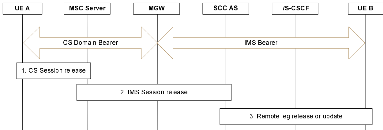
Figure 7.7.2.2-1: Session Release initiated by UE A when using an MSC server enhanced for ICS
