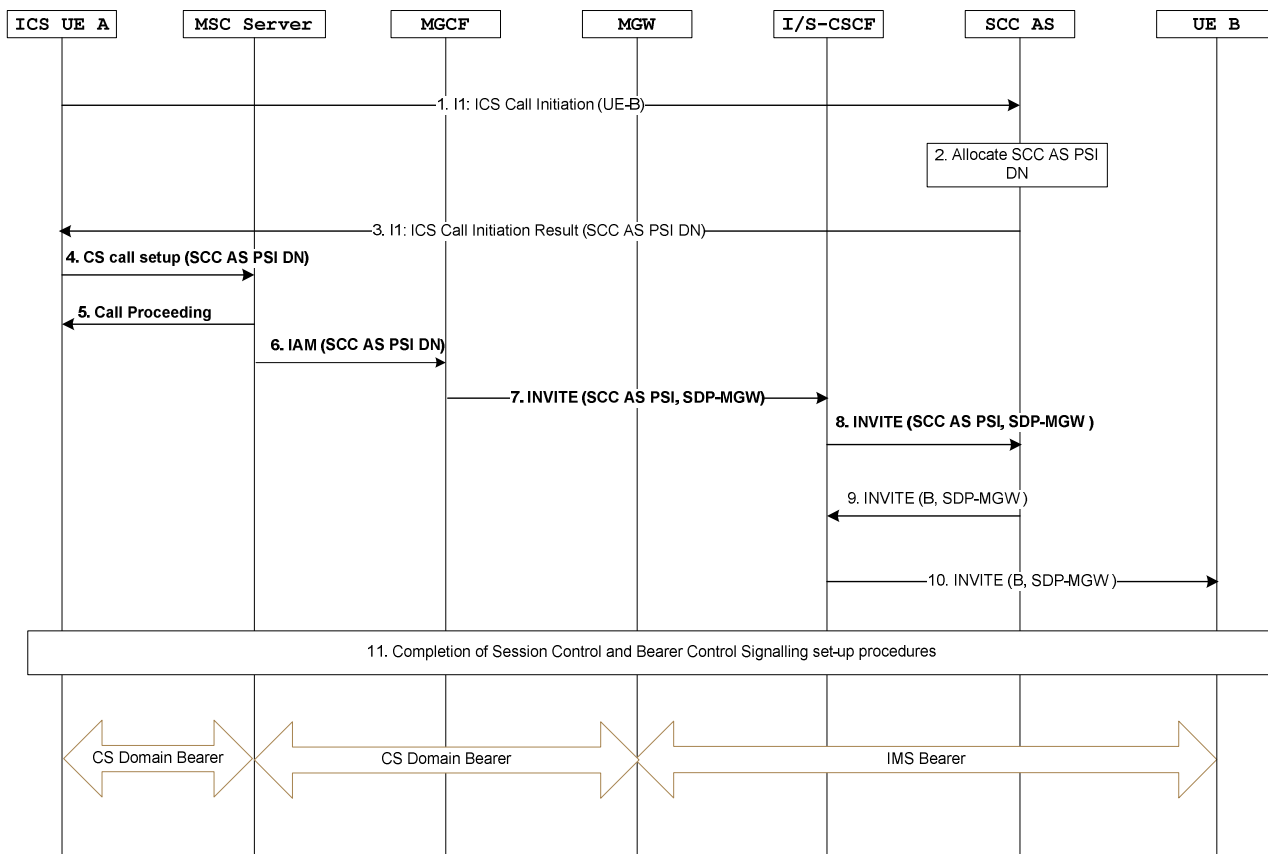
Figure 7.3.2.2.2.1-2: ICS UE Origination with CS media addressing a SIP-URI when using an MSC Server
