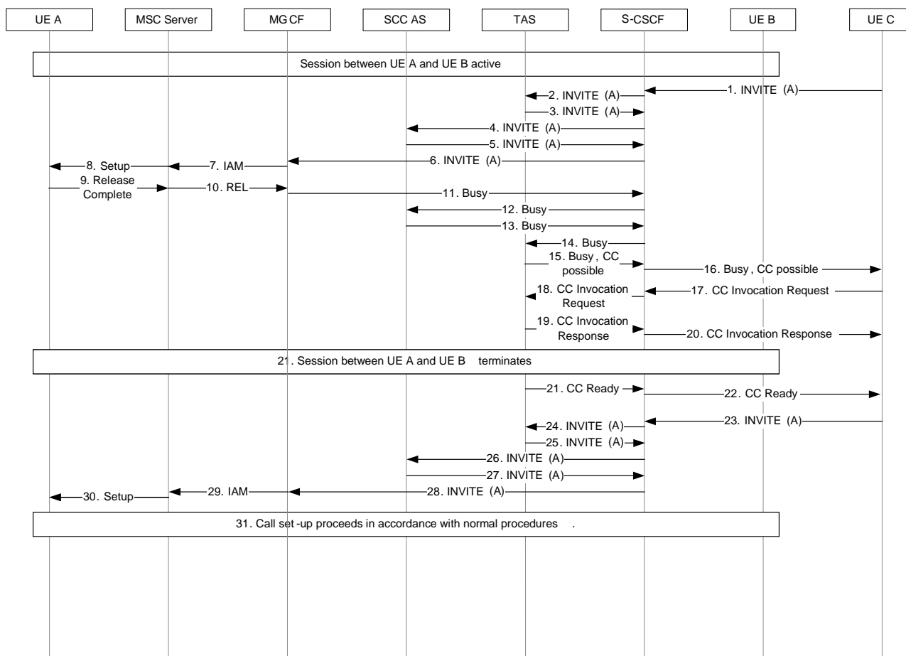
Figure 7.6.3.10.1-1: IMS Communication Completion to Busy Subscriber via MSC Server not enhanced for ICS
