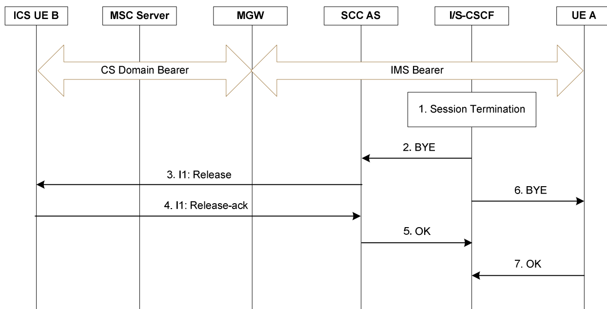
Figure 7.7.1.3.2-1: Network initiated release of a service control signalling session initiated using I1
