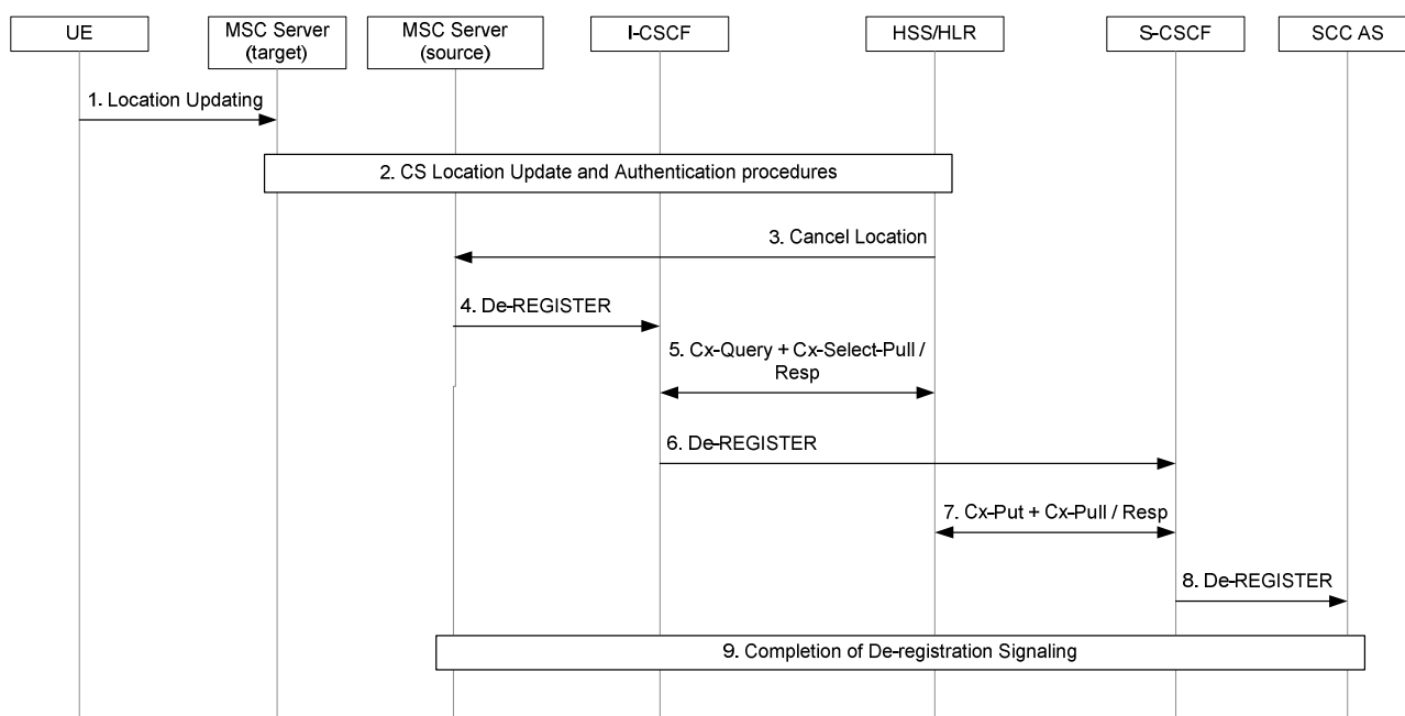
Figure 7.2.1.3-1: IMS Deregistration via CS Access by source MSC Server enhanced for ICS when moving to an MSC Server not enhanced for ICS
