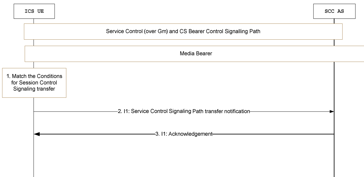
Figure 7.8-1: Service Control Signaling Path handover from Gm to I1
