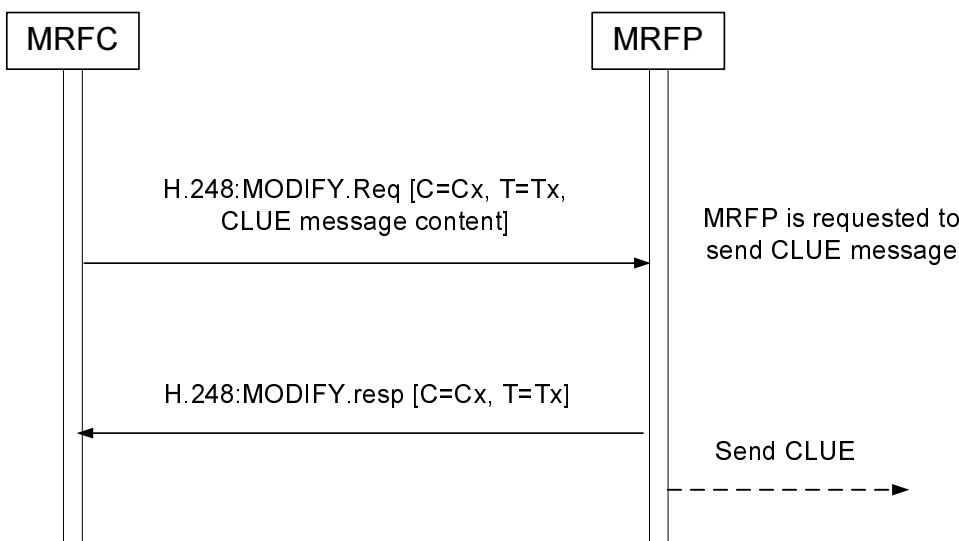
Figure 6.2.21.2.2: Procedure for sending CLUE message
