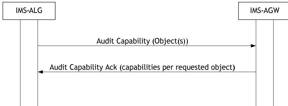
Figure 6.1.8.2.1: Audit Capability
