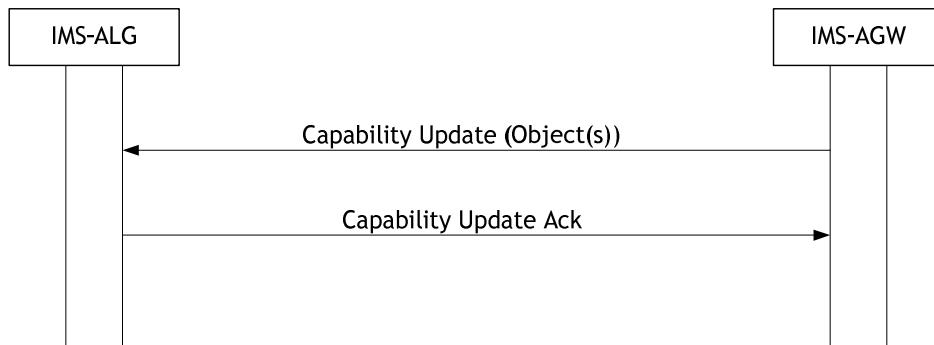
Figure 6.1.9.1: Capability Update
