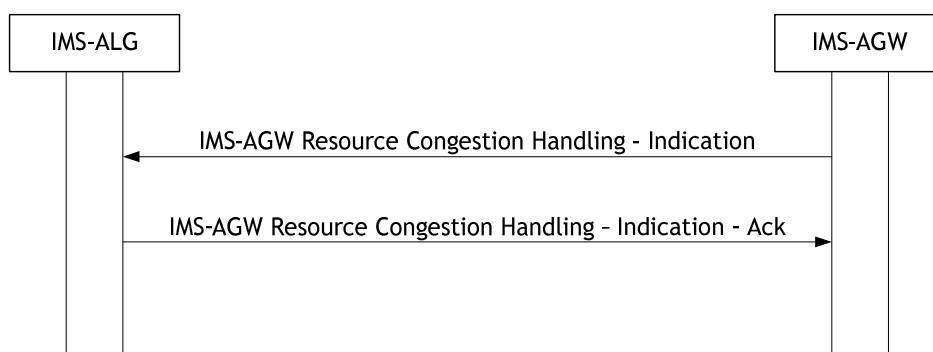
Figure 6.1.12.1: IMS-AGW Resource Congestion Handling – Indication
