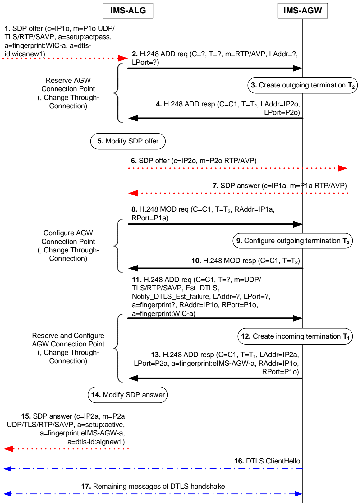
Figure 6.2.10.5.1: WIC originated procedure using DTLS-SRTP
