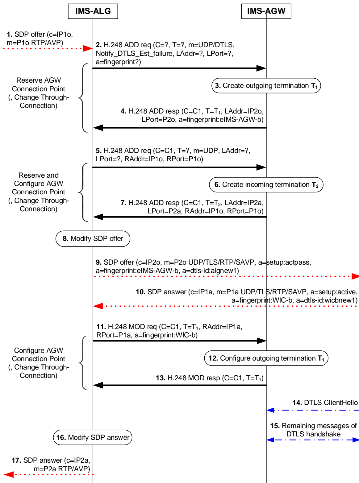
Figure 6.2.10.5.2: WIC terminated procedure using DTLS-SRTP
