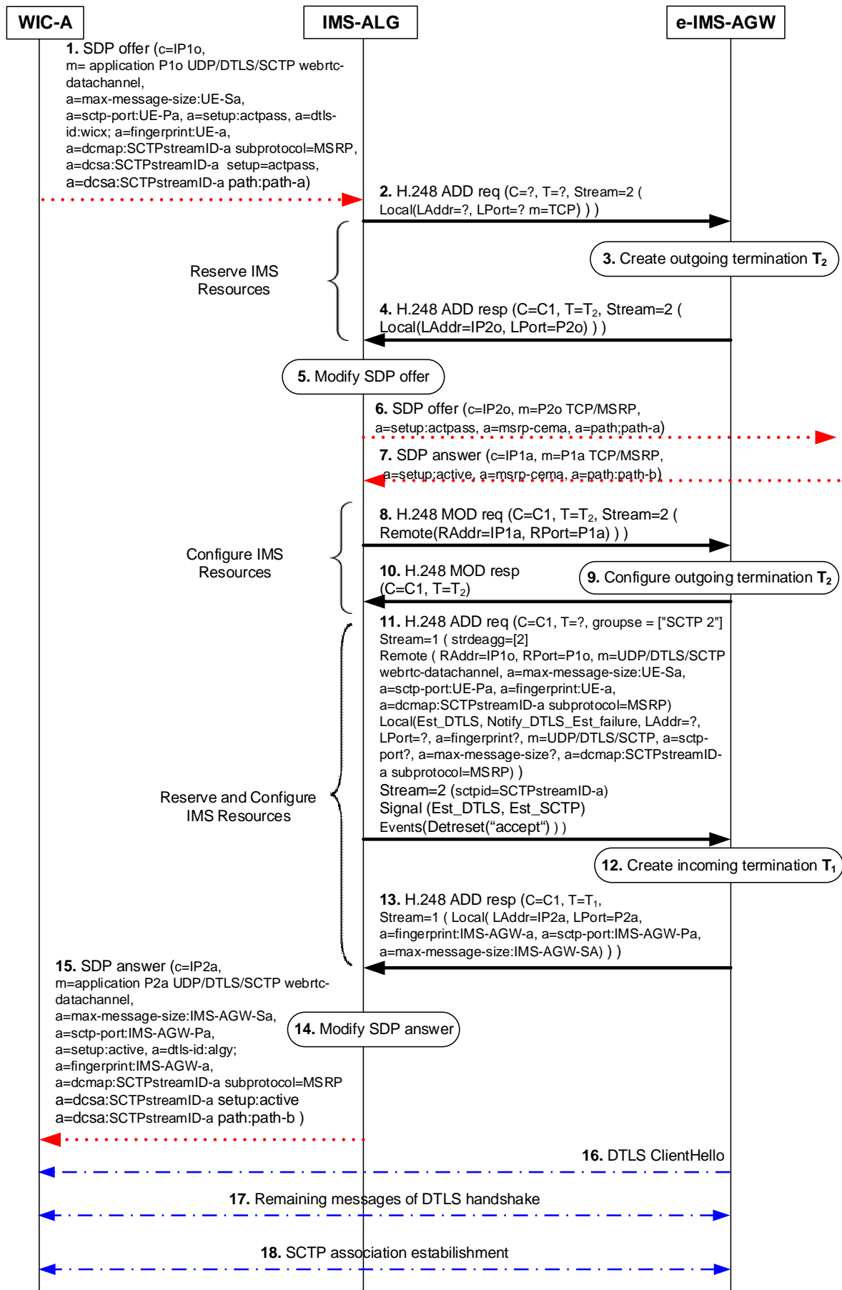
Figure 6.2.10.6.2.2: WIC originated procedure for WebRTC data channel establishment and MSRP stream establishment
