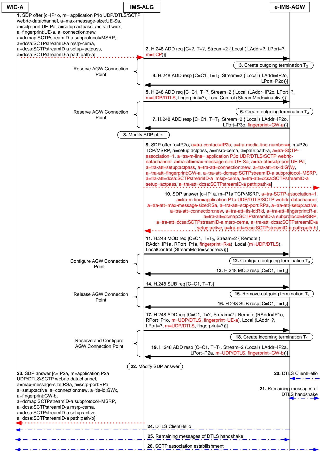
Figure 6.2.23.2.1: WIC originated procedure for WebRTC data channel establishment with media plane optimization excluding DTLS layer
