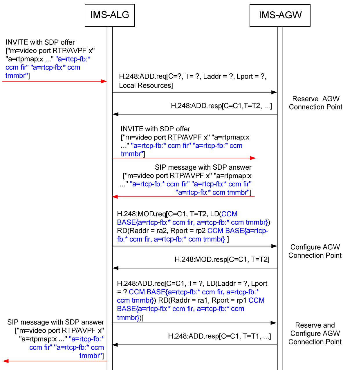
Figure 6.2.24.1: Procedure to indicate RTCP Codec Control Commands and Indications
