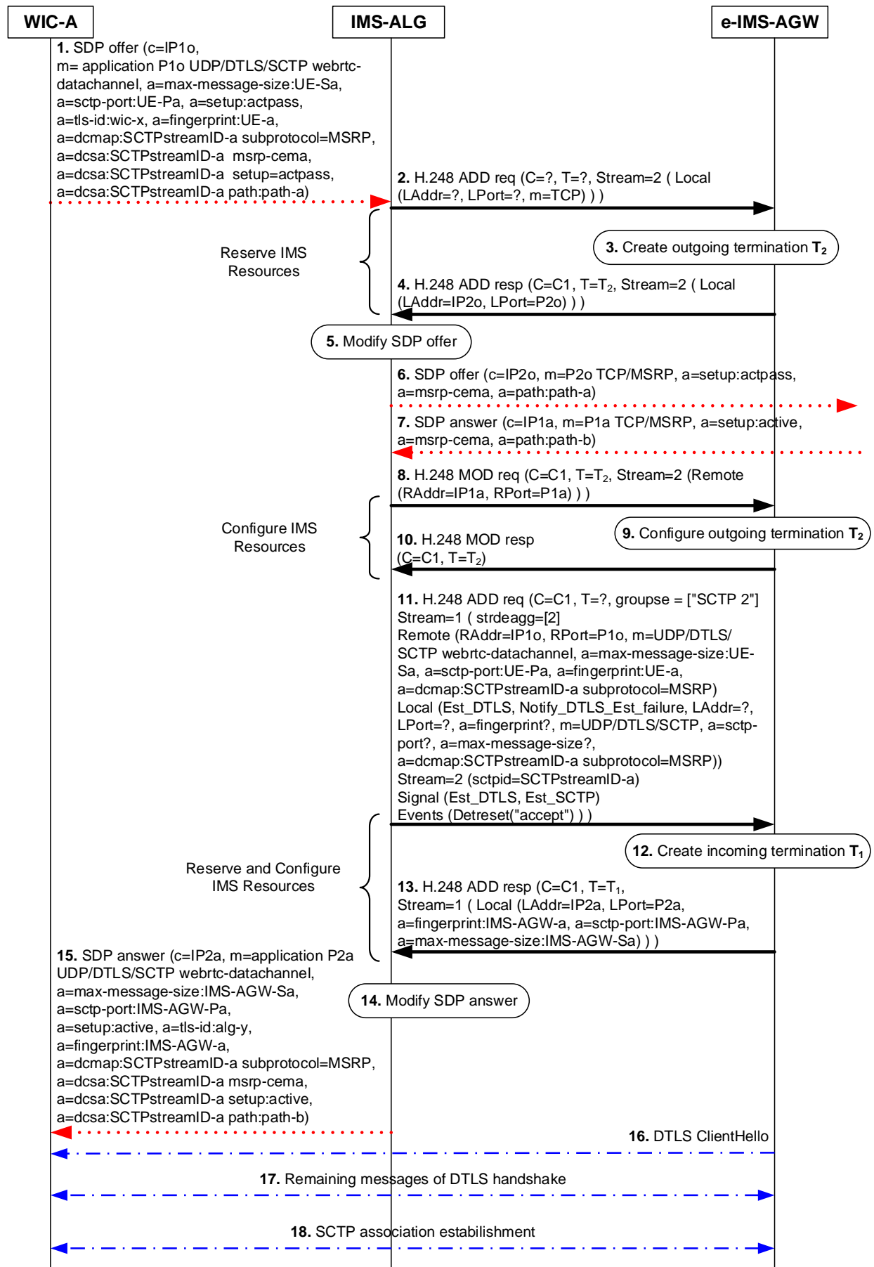
Figure 6.2.10.6.2.2: WIC originated procedure for WebRTC data channel establishment and MSRP stream establishment
