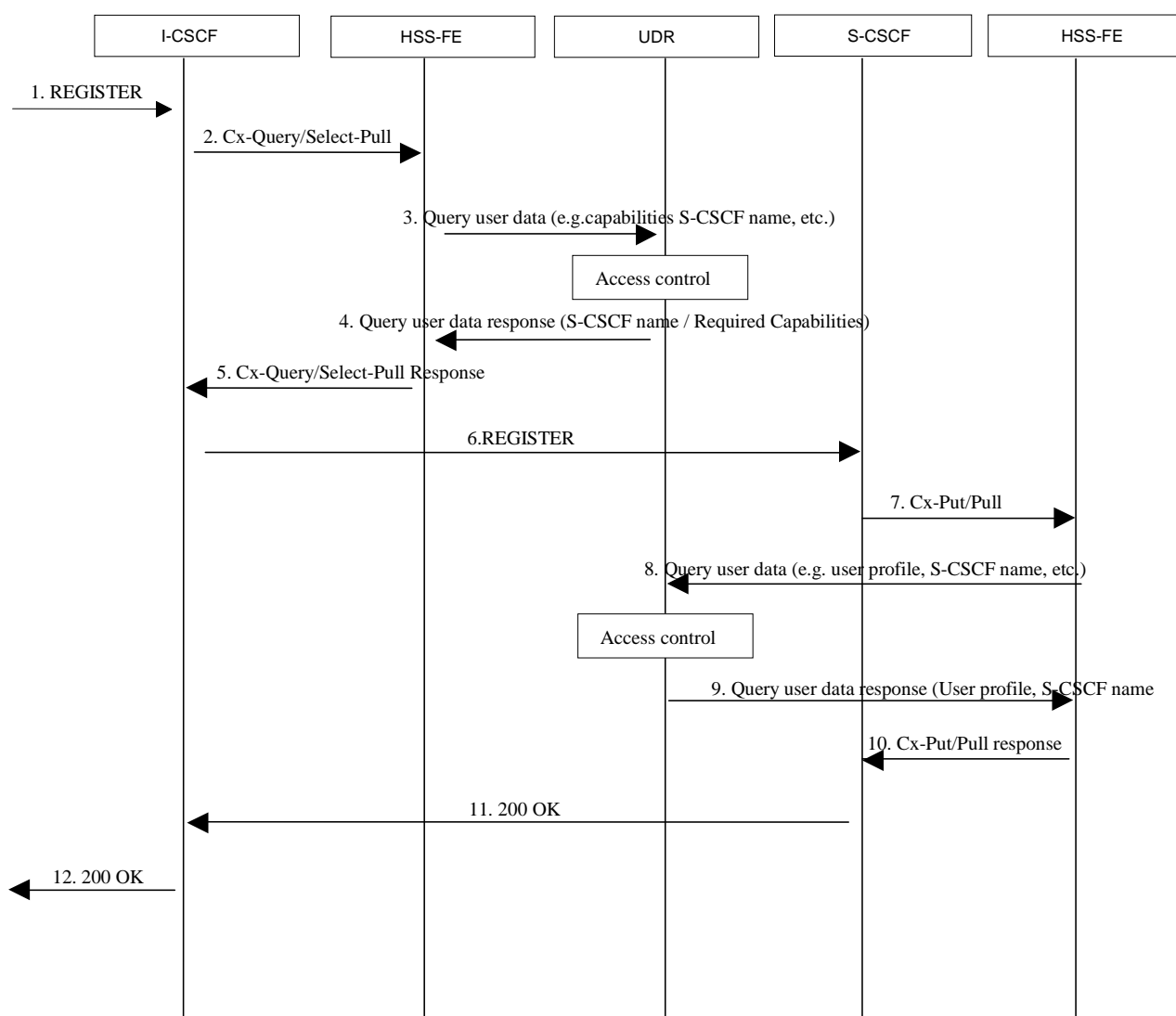
Figure A.1.3-1: IMS re-registration flow example with Udr Query from HSS-FE
