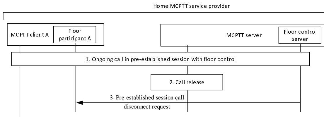
Figure 10.5.3.2.2-1: Disconnect procedure
