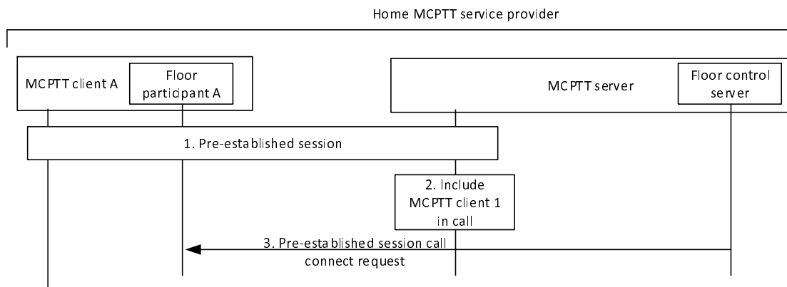
Figure 10.5.3.2.1-1: Connect procedure
