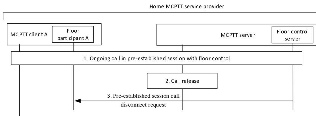
Figure 10.5.3.2.2-1: Disconnect procedure
