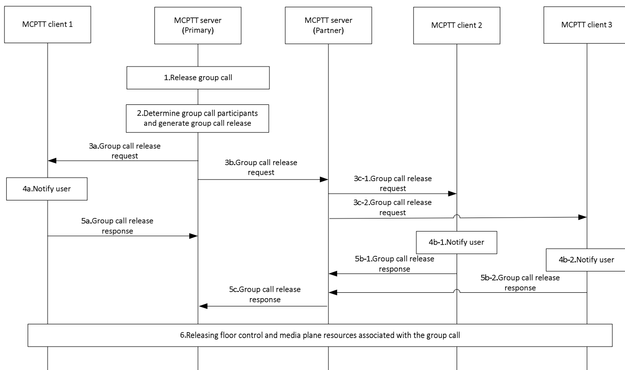
Figure 10.6.2.4.1.2-1: Group call release involving groups from multiple MCPTT systems
