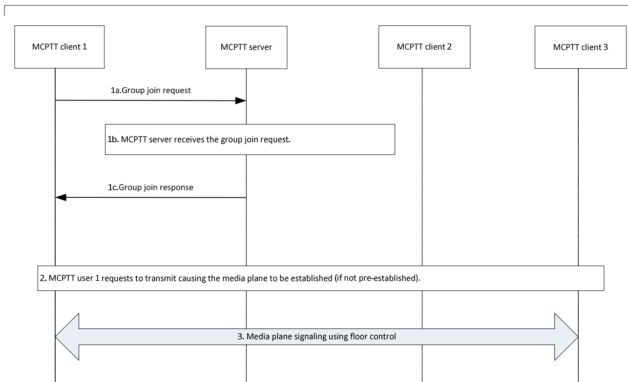
Figure 10.6.2.3.1.2.2-1: MCPTT chat group call
