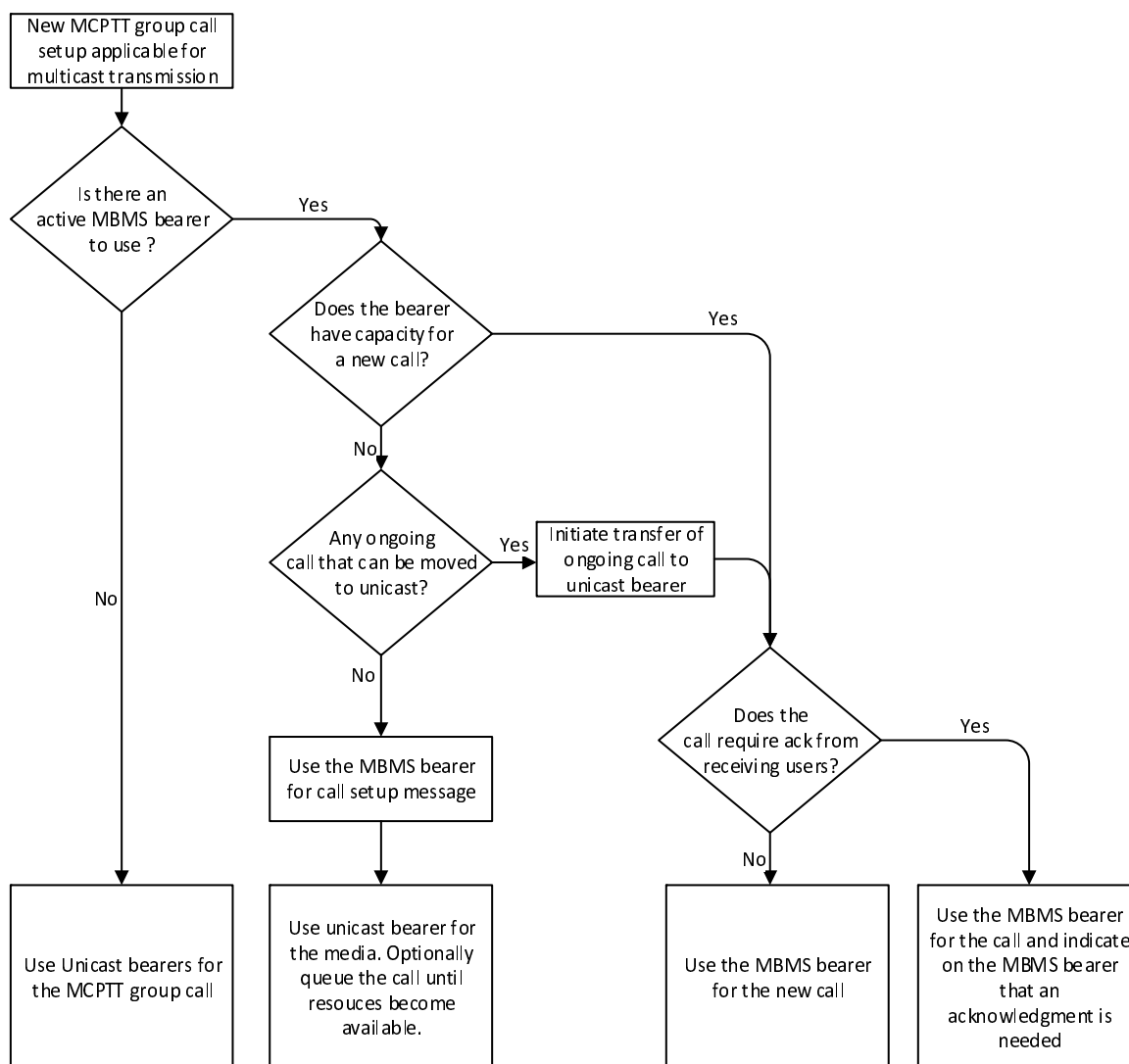
Figure 10.10.6.1-1: MBMS bearer decision flow
