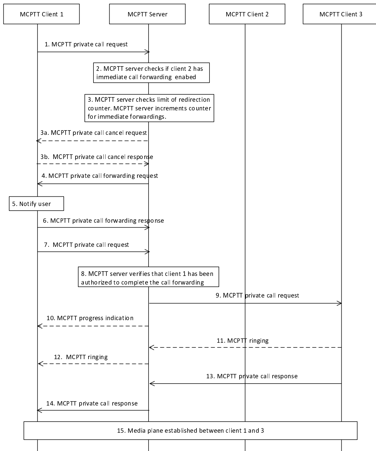
Figure 10.7.5.2.2-1: Call forwarding immediate for private calls
