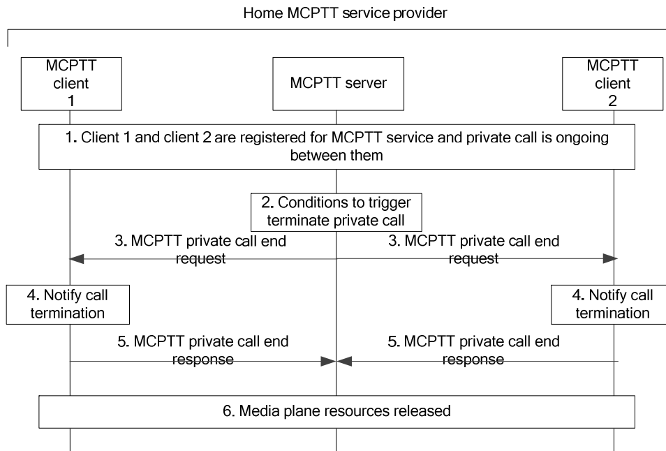
Figure 10.7.2.3.2-1: End private call – server initiated
