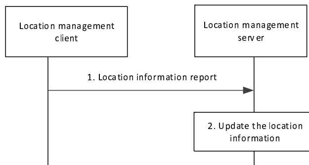
Figure 9.3.3.3-1: Location reporting procedure
