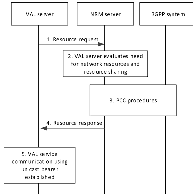
Figure 14.3.3.3.2-1: Resource request at VAL service communication establishment
