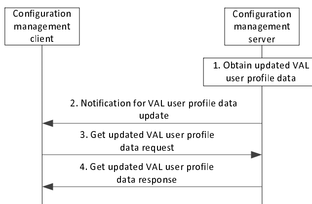
Figure 11.3.4.3-1: VAL user receives updated VAL user profile data from the network
