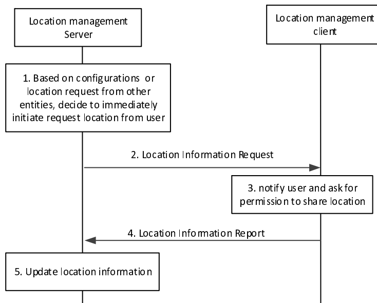
Figure 9.3.4-1: On-demand location information reporting procedure
