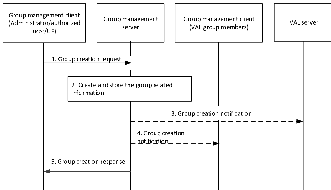
Figure 10.3.3-1: Group creation
