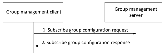
Figure 10.3.6.3-1: Subscription for group configurations
