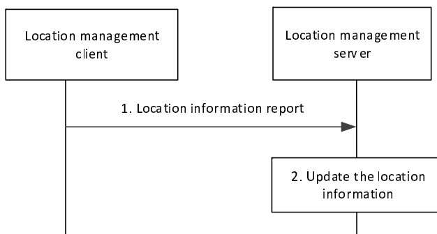
Figure 9.3.3-1: Location reporting procedure
