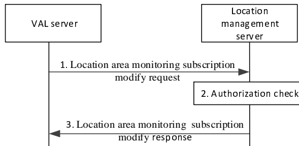
Figure 9.3.12.2-1: Location area monitoring subscription modify procedure
