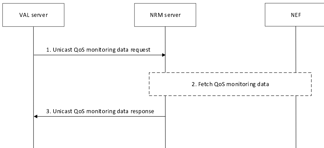
Figure 14.3.3.4.4.2-1: Retrieval of unicast QoS monitoring data
