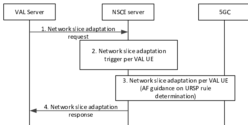
Figure 16.3.2.3-1: Network slice adaptation for VAL application
