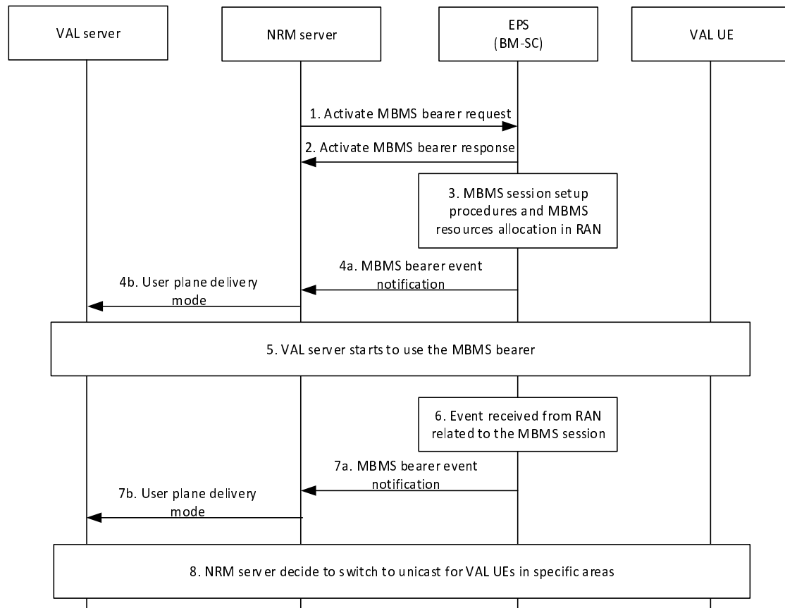
Figure 14.3.4.8.2-1: MBMS bearer event notification
