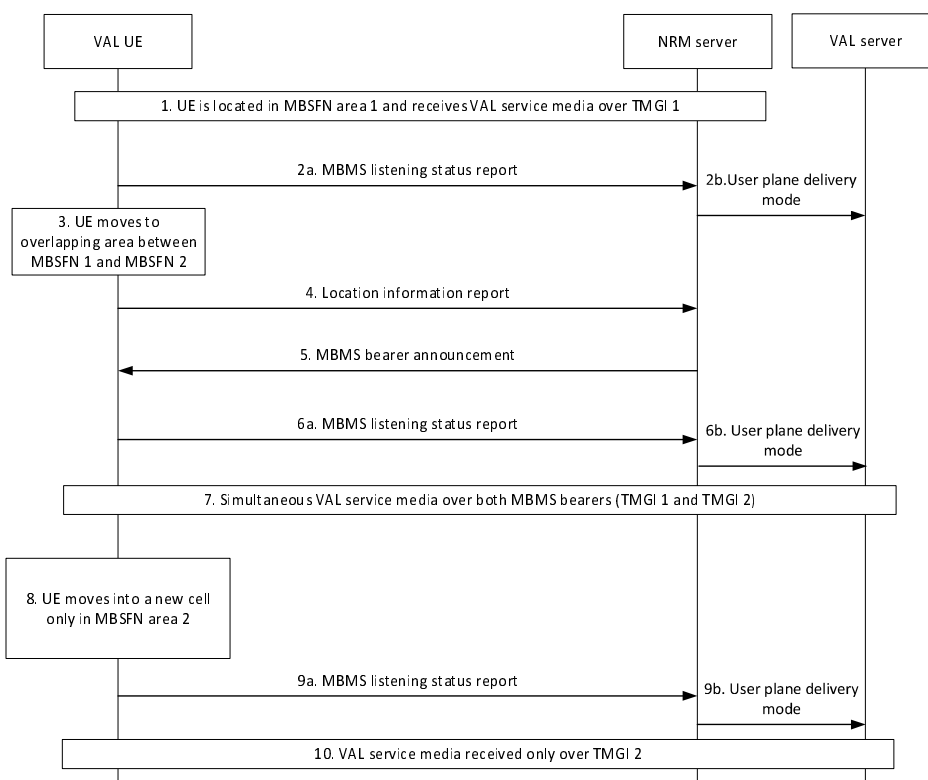
Figure 14.3.4.6.2-2: Service continuity when moving from one MBSFN to another
