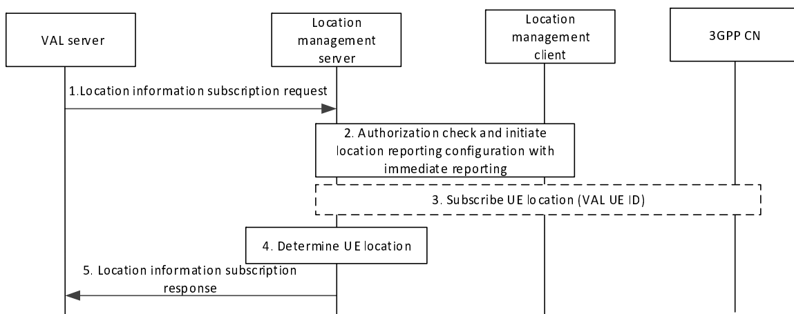
Figure 9.3.7-1: Location information subscription request procedure
