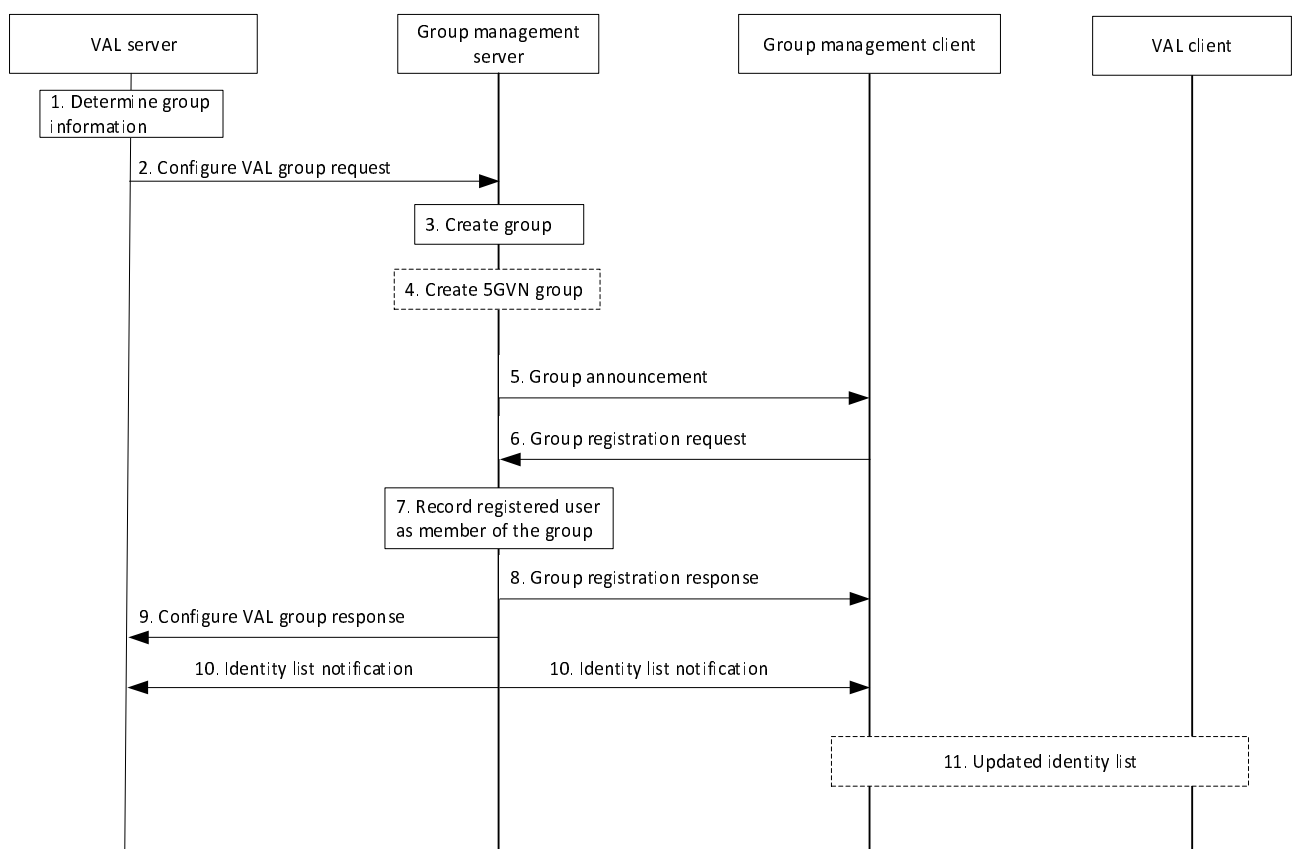
Figure 10.3.8.2-1: Procedure for establishing VAL group communication between the group management server and group management client1.
