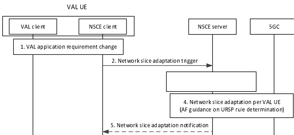
Figure 16.3.2.4-1: Network slice adaptation for VAL application
