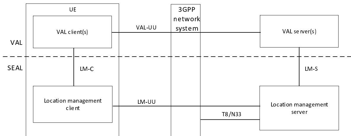
Figure 9.2.2-1: On-network functional model for location management
