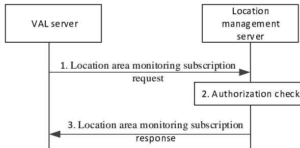
Figure 9.3.12.1-1: Location area monitoring subscription procedure
