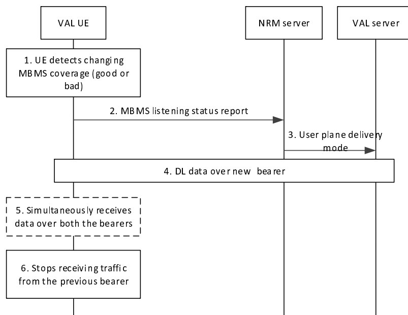
Figure 14.3.4.9.2-1: Switching between MBMS delivery and unicast delivery
