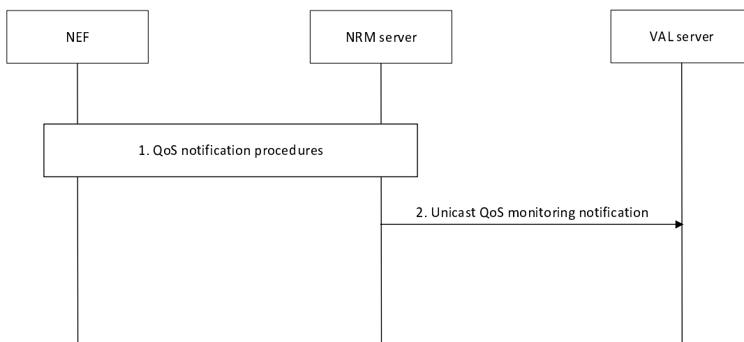
Figure 14.3.3.4.2.2-1: Unicast QoS monitoring notification procedure
