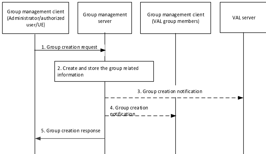
Figure 10.3.3-1: Group creation
