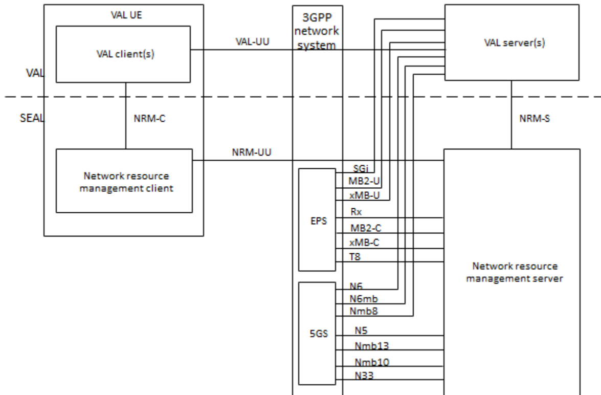
Figure 14.2.2.1-1: On-network functional model for network resource management
