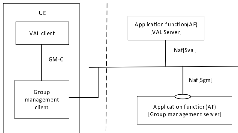
Figure 10.2.2-2: Architecture for group management – Service based representation
