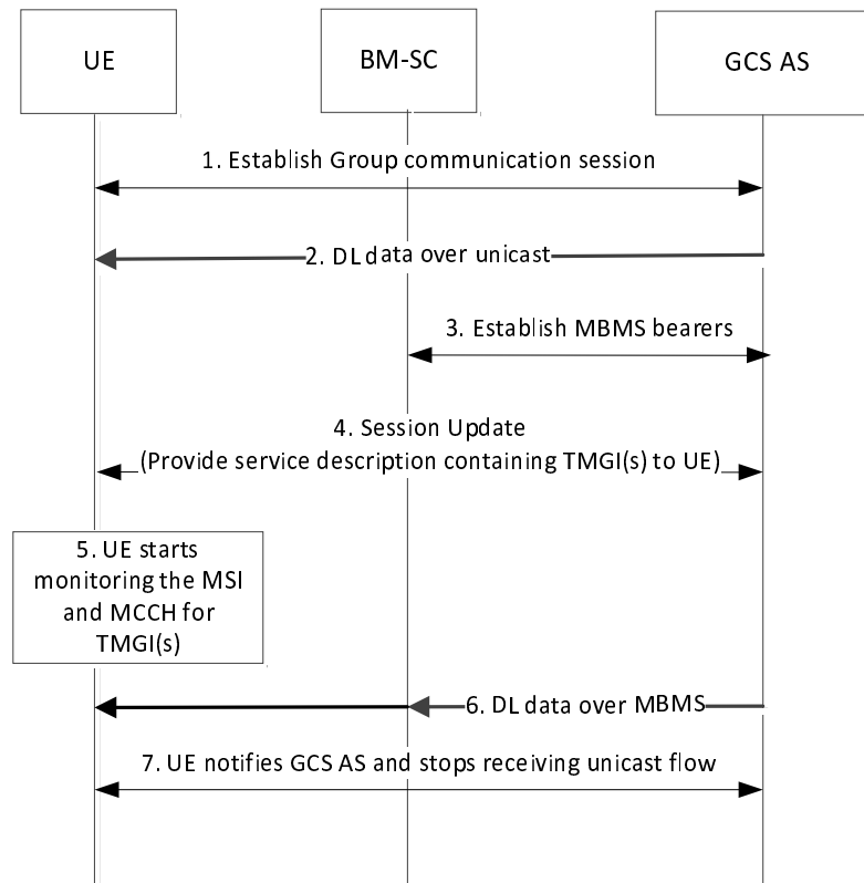
Figure A.2.3-1: Use of Dynamic MBMS Bearer Establishment
