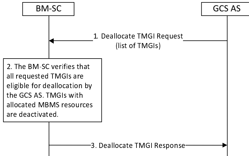
Figure 5.1.2.2-1: TMGI Deallocation Procedure
