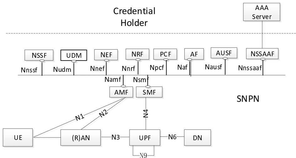
Figure 5.30.2.9.2-1: 5G System architecture with access to SNPN using credentials from Credentials Holder using AAA Server
