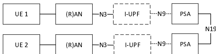
Figure 4.4.6.1-2: N19-based user plane architecture in non-roaming scenario
