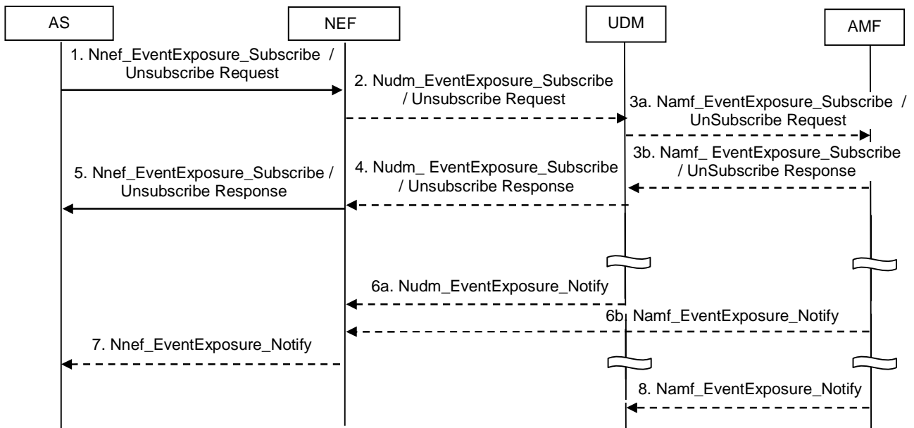
Figure 4.15.3.2.3-1: Nnef_EventExposure_Subscribe, Unsubscribe and Notify operations
