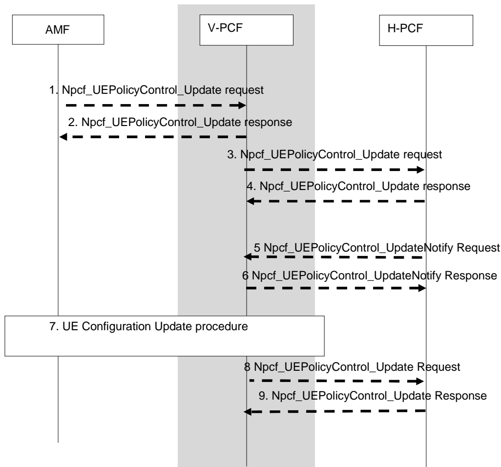
Figure 4.16.12.1-1: UE Policy Association Modification initiated by the AMF
