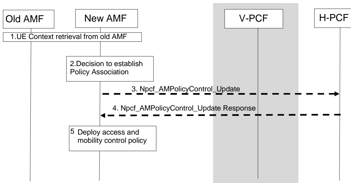
Figure 4.16.2.1.2-1: Policy Association Modification with the old PCF during AMF relocation
