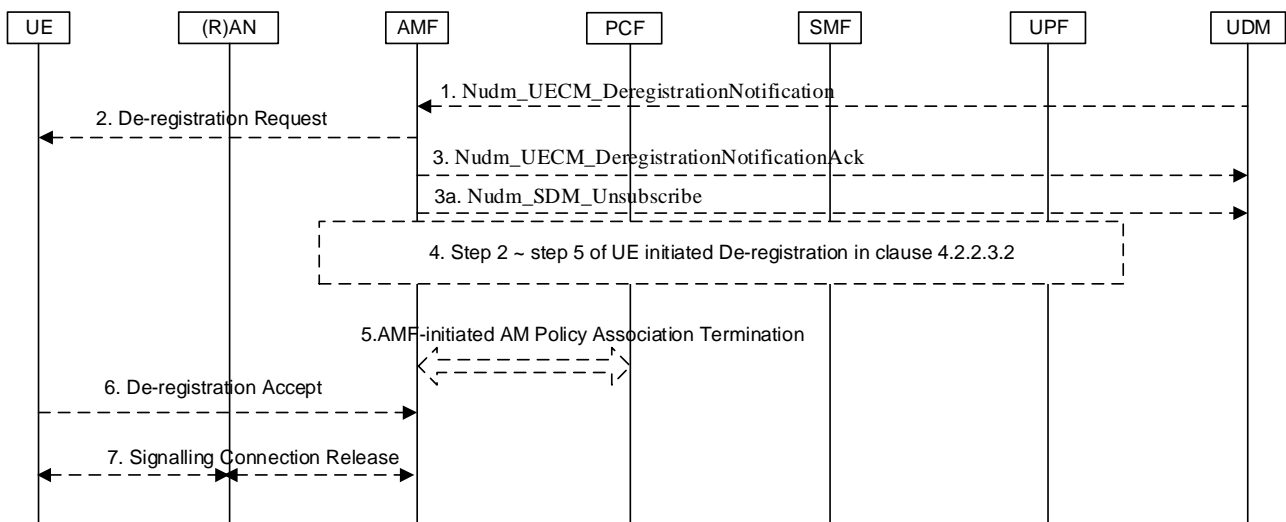
Figure 4.2.2.3.3-1: Network-initiated Deregistration
