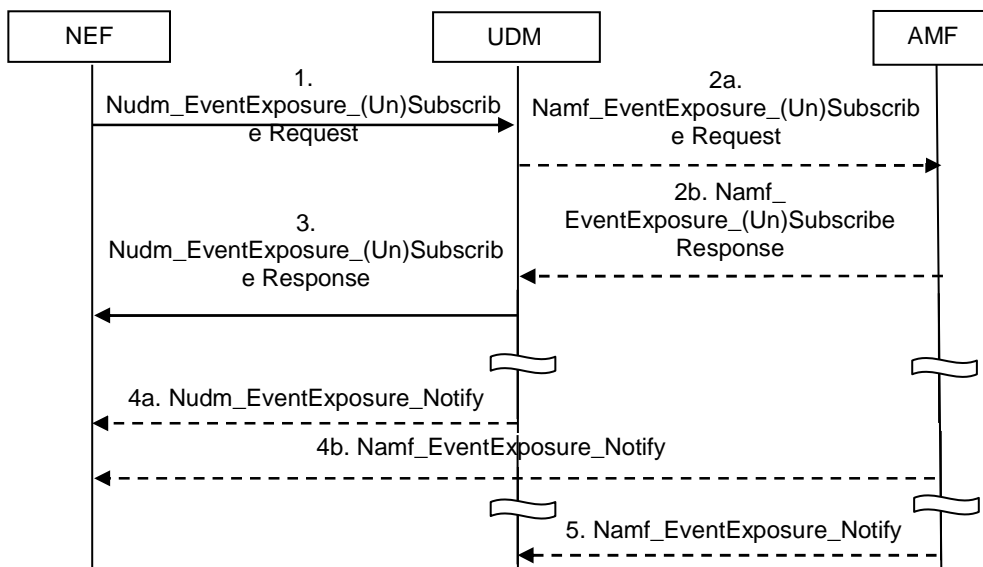
Figure 4.15.3.2.2-1: Nudm_EventExposure_Subscribe, Unsubscribe and Notify operations
