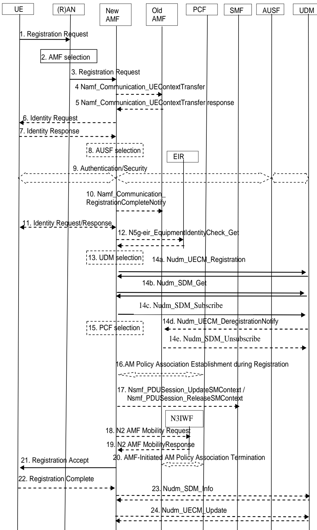
Figure 4.2.2.2.2-1: Registration procedure
