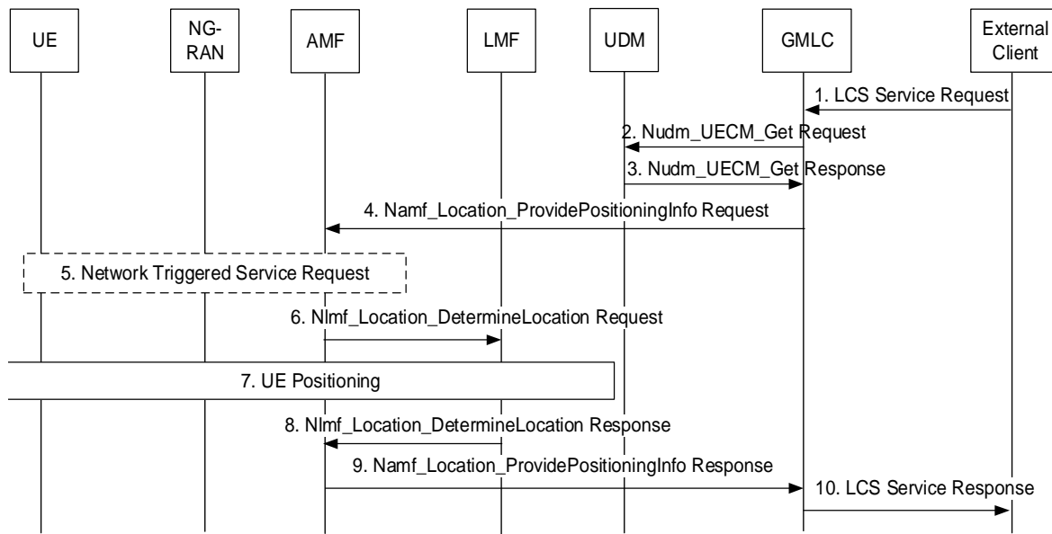
Figure 4.13.5.3-1: 5GC-MT-LR Procedure
