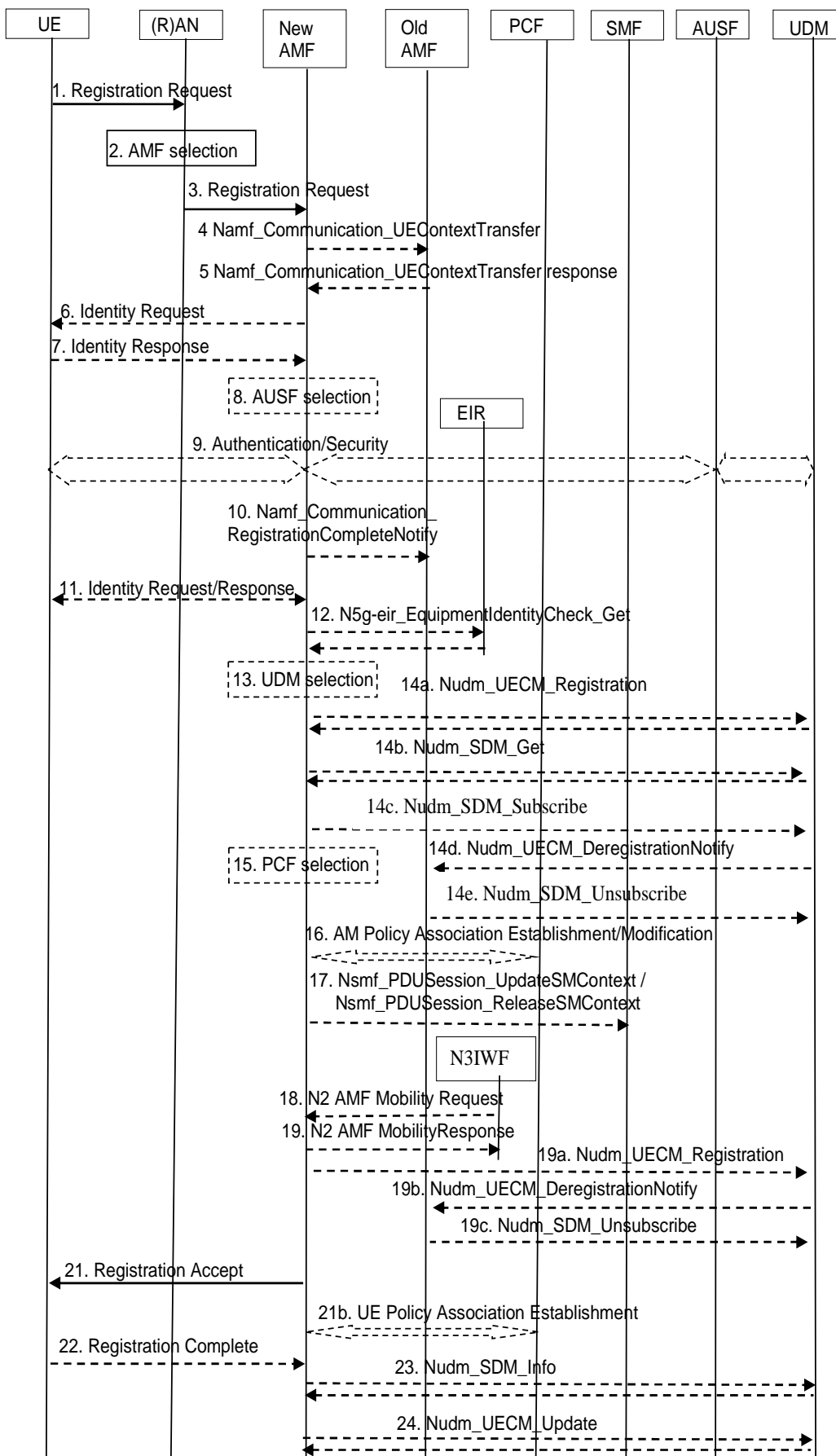
Figure 4.2.2.2-1: Registration procedure
