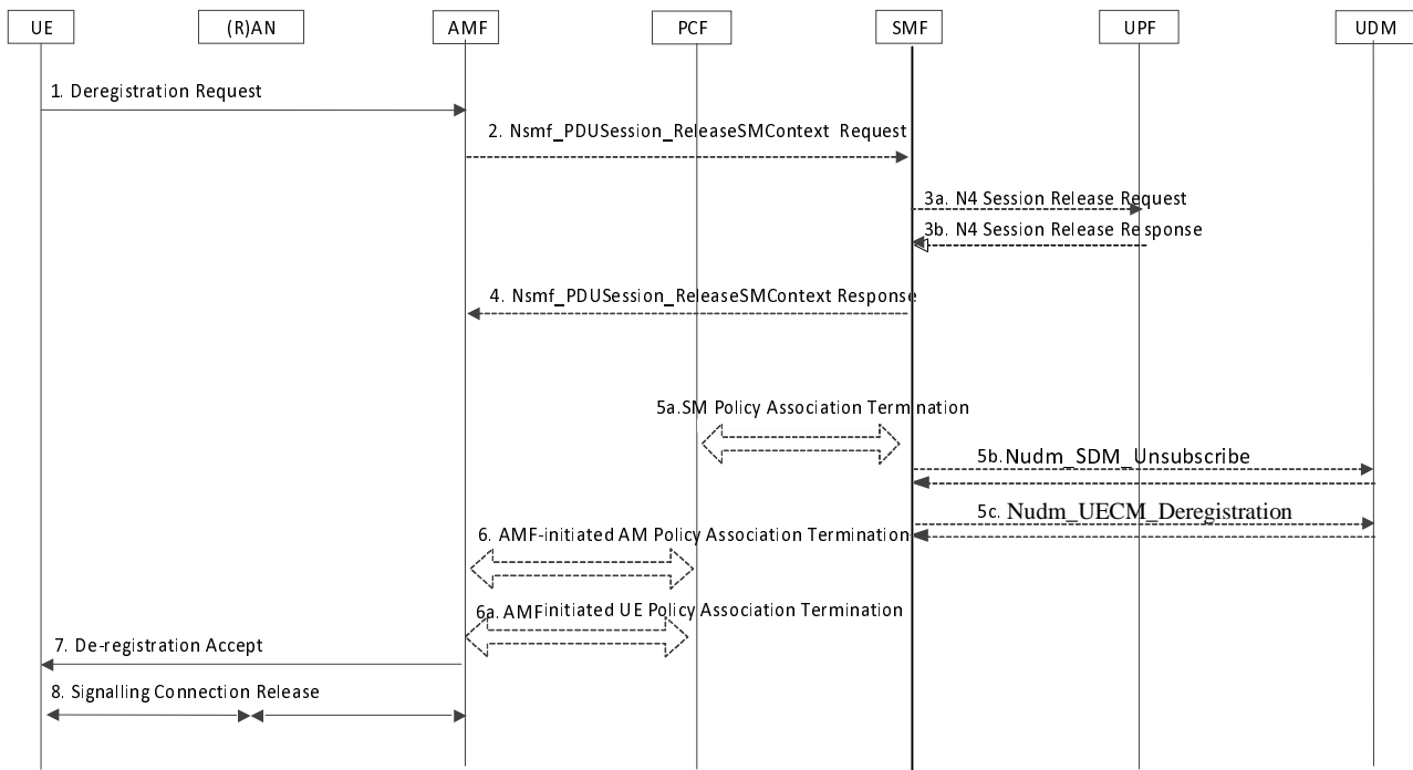
Figure 4.2.3.2-1: UE-initiated Deregistration
