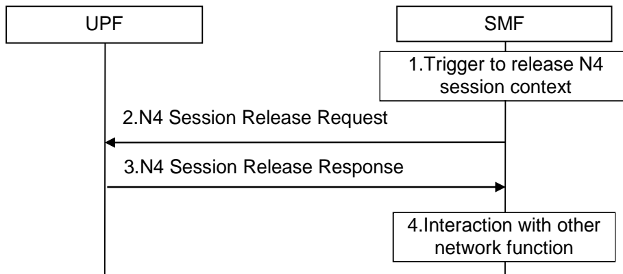
Figure 4.4.1.4-1 N4 Session Release procedure
