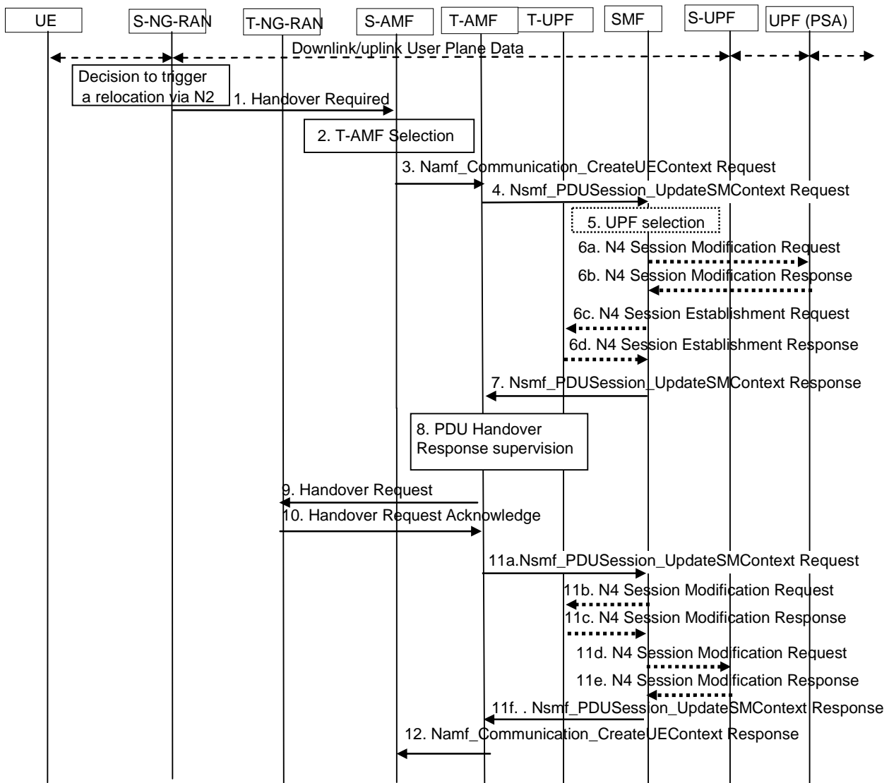
Figure 4.9.1.3.2-1: Inter NG-RAN node B2 based handover, Preparation phase
