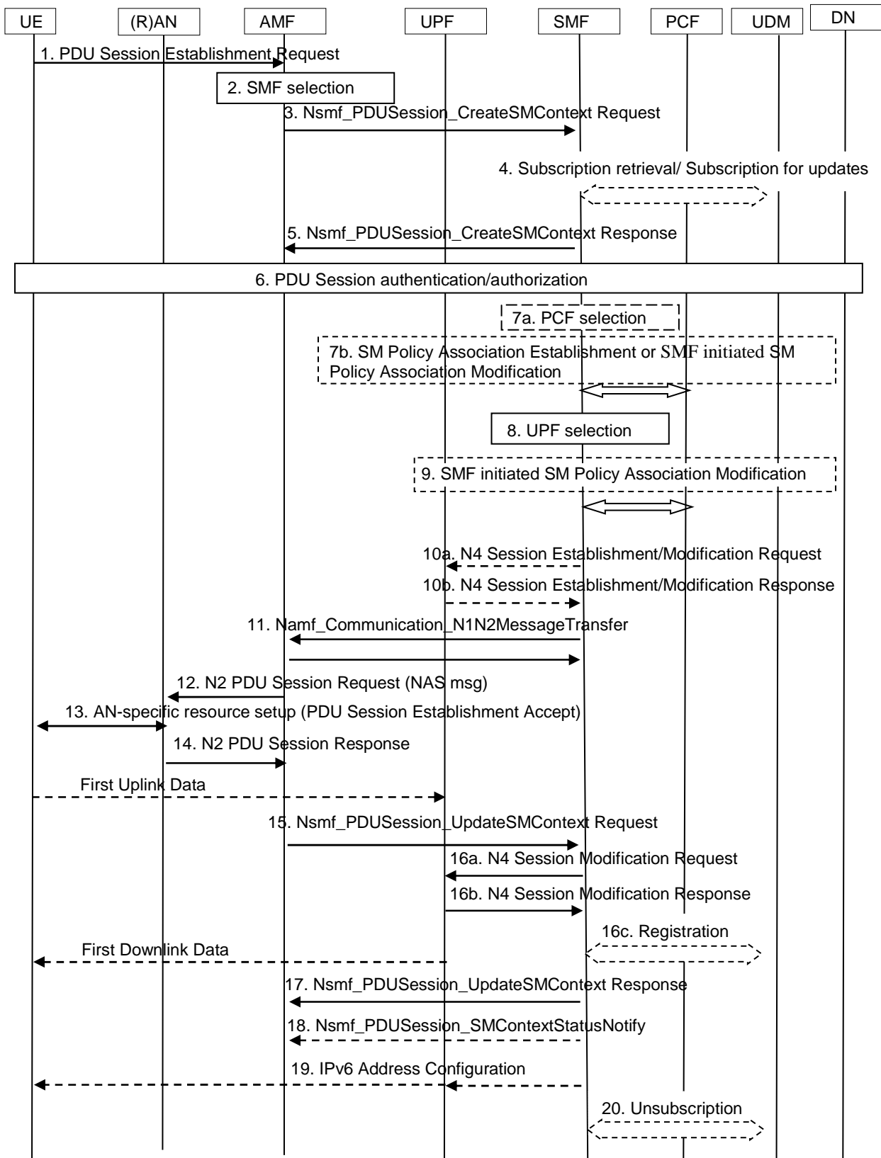
Figure 4.3.2.1-1: UE-requested PDU Session Establishment for non-roaming and roaming with local breakout
