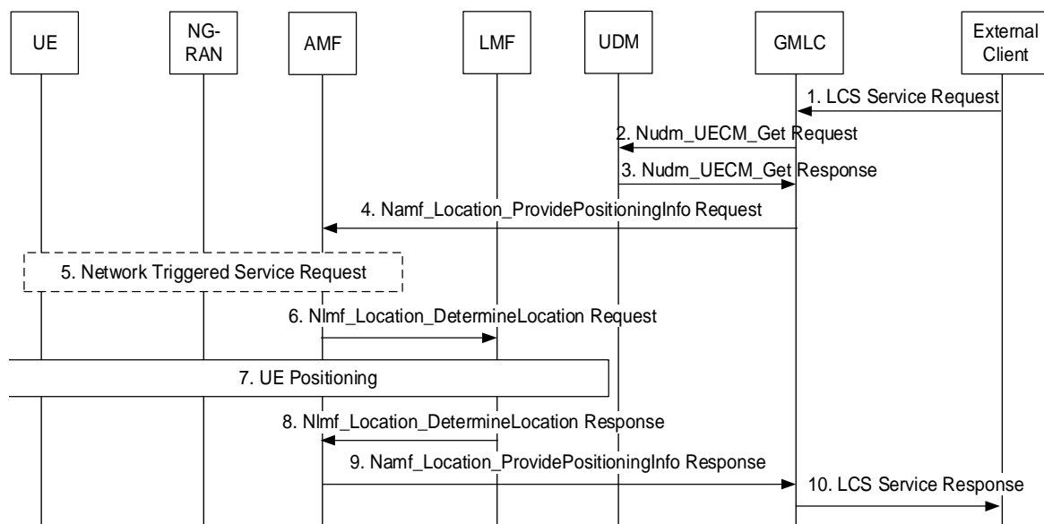
Figure 4.13.5.3-1: 5GC-MT-LR Procedure
