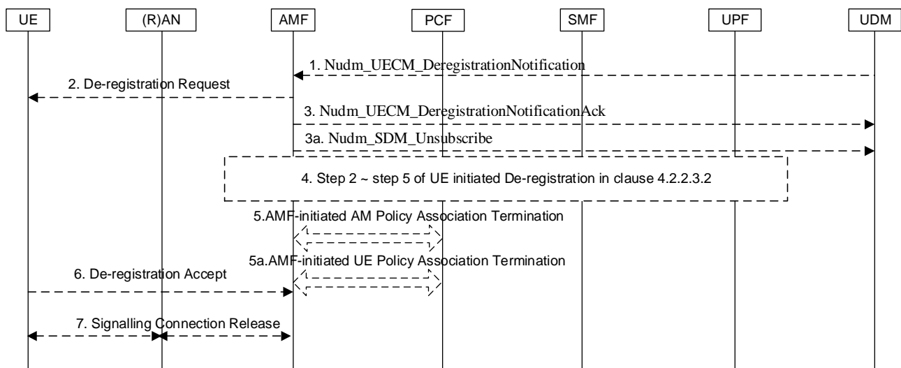
Figure 4.2.2.3.3-1: Network-initiated Deregistration
