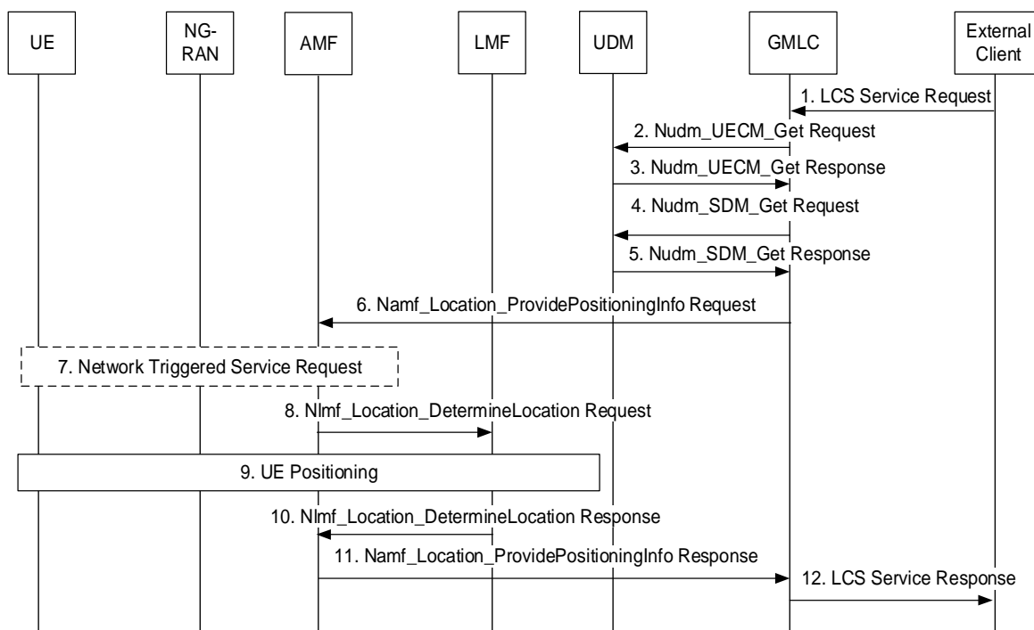
Figure 4.13.5.3-1: 5GC-MT-LR Procedure
