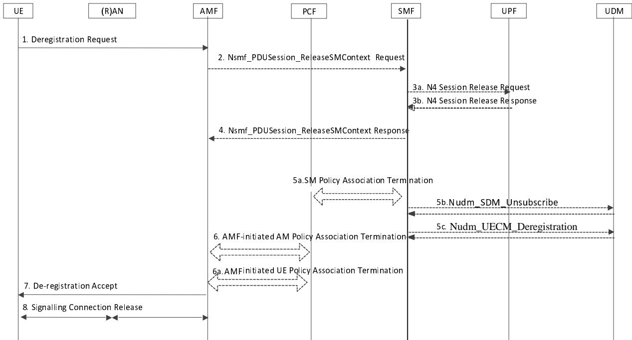
Figure 4.2.2.3.2-1: UE-initiated Deregistration
