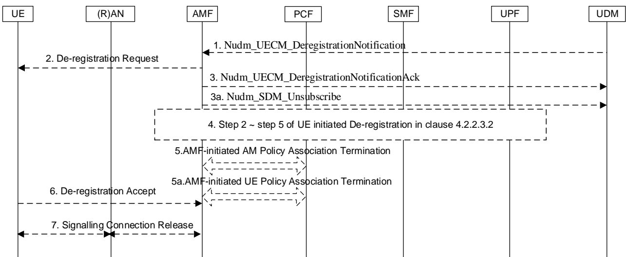
Figure 4.2.2.3.3-1: Network-initiated Deregistration
