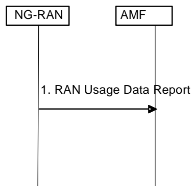
Figure 4.21-1: RAN Secondary RAT Usage Data Reporting procedure
