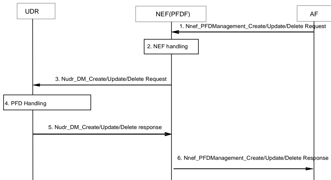
Figure 4.18.2-1 procedure for PFD management via NEF (PFDF)
