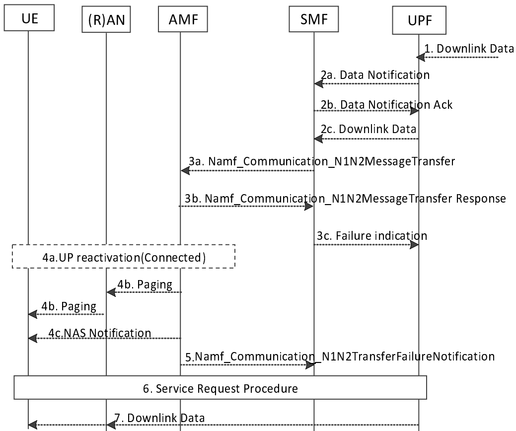
Figure 4.2.3.3-1: Network Triggered Service Request
