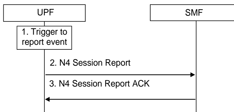
Figure 4.4.2.2-1: N4 Session Level Reporting procedure
