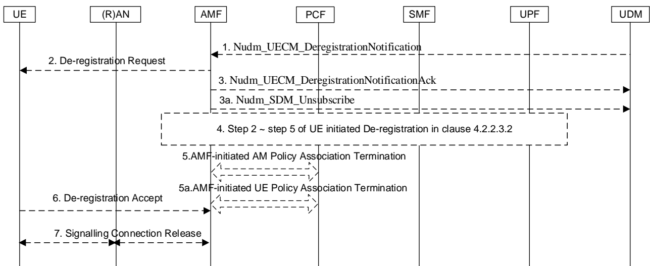
Figure 4.2.2.3.3-1: Network-initiated Deregistration
