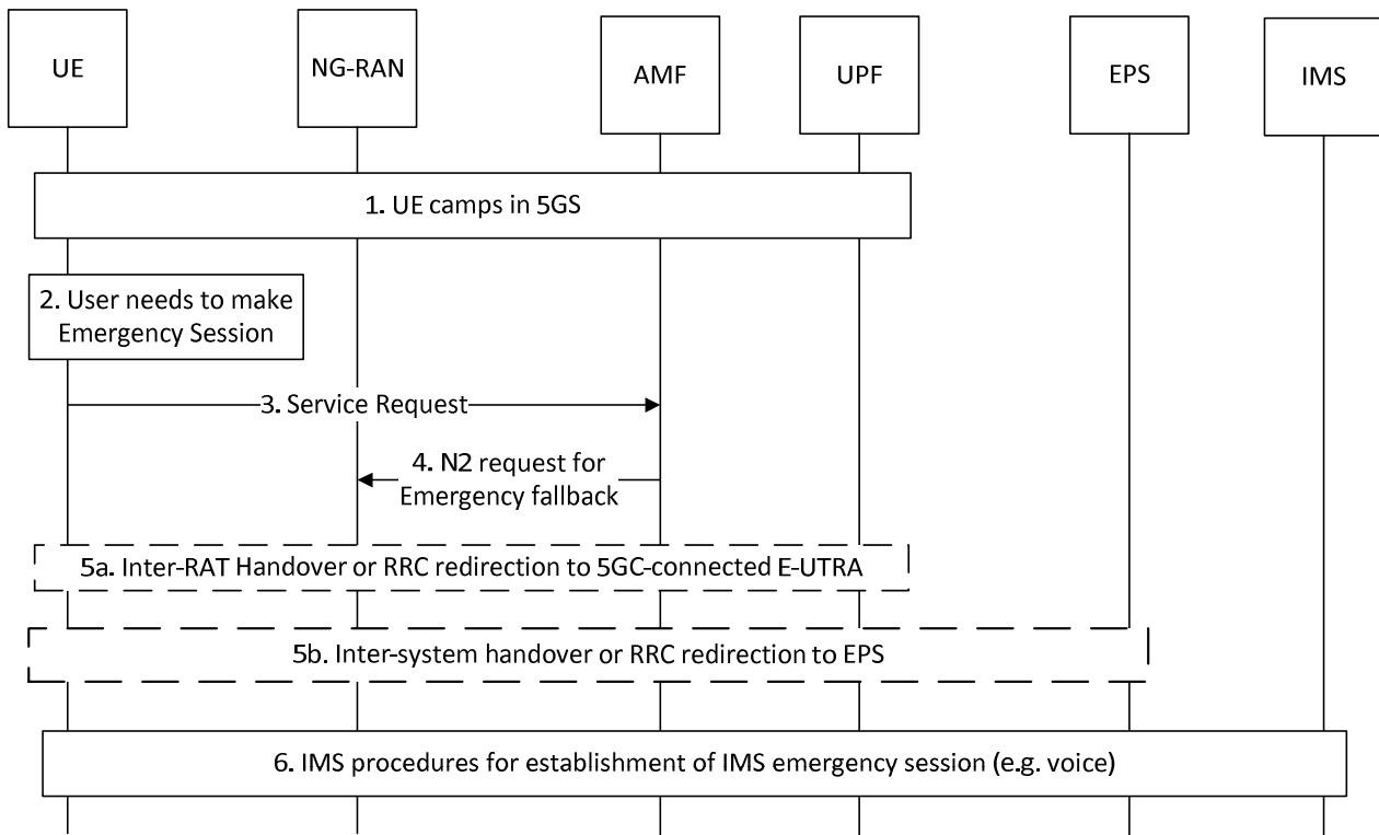
Figure 4.13.4.2-1: Emergency Services Fallback
