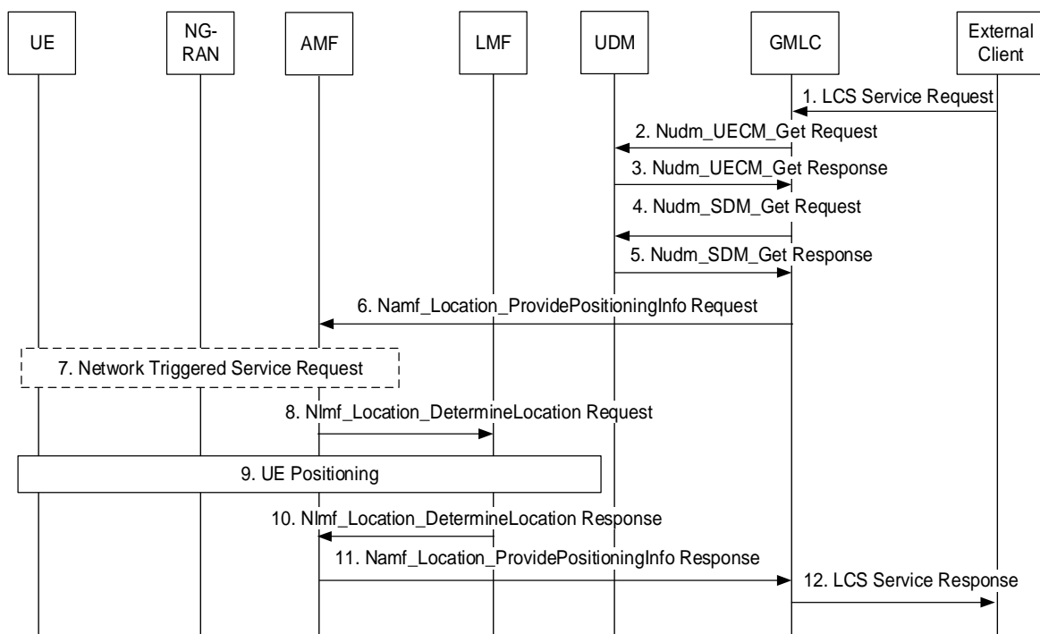
Figure 4.13.5.3-1: 5GC-MT-LR Procedure
