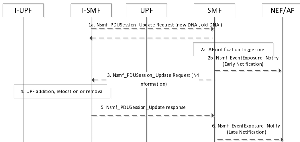
Figure 4.23.6.3-1: Reporting UP path change to the AF
