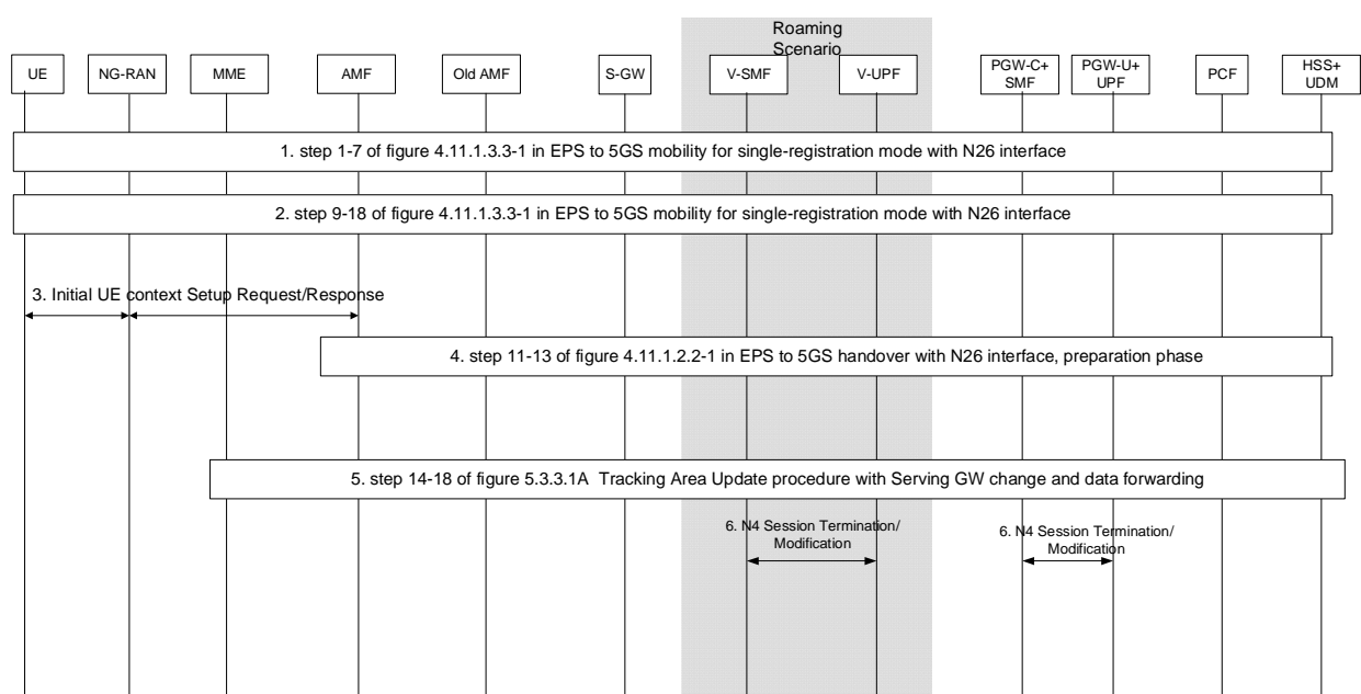
Figure 4.11.1.3.3A-1: EPS to 5GS Idle mode mobility using N26 interface with data forwarding
