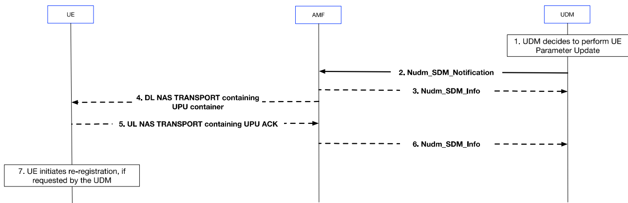
Figure 4.20.2-1: UE Parameters Update via UDM Control Plane Procedure
