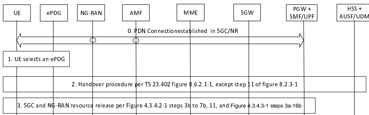
Figure 4.11.4.2-1: Handover from 5GS to EPC/ePDG
