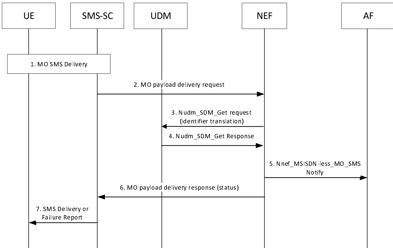
Figure 4.13.7.2-1: MSISDN-less MO SMS procedure via Nnef
