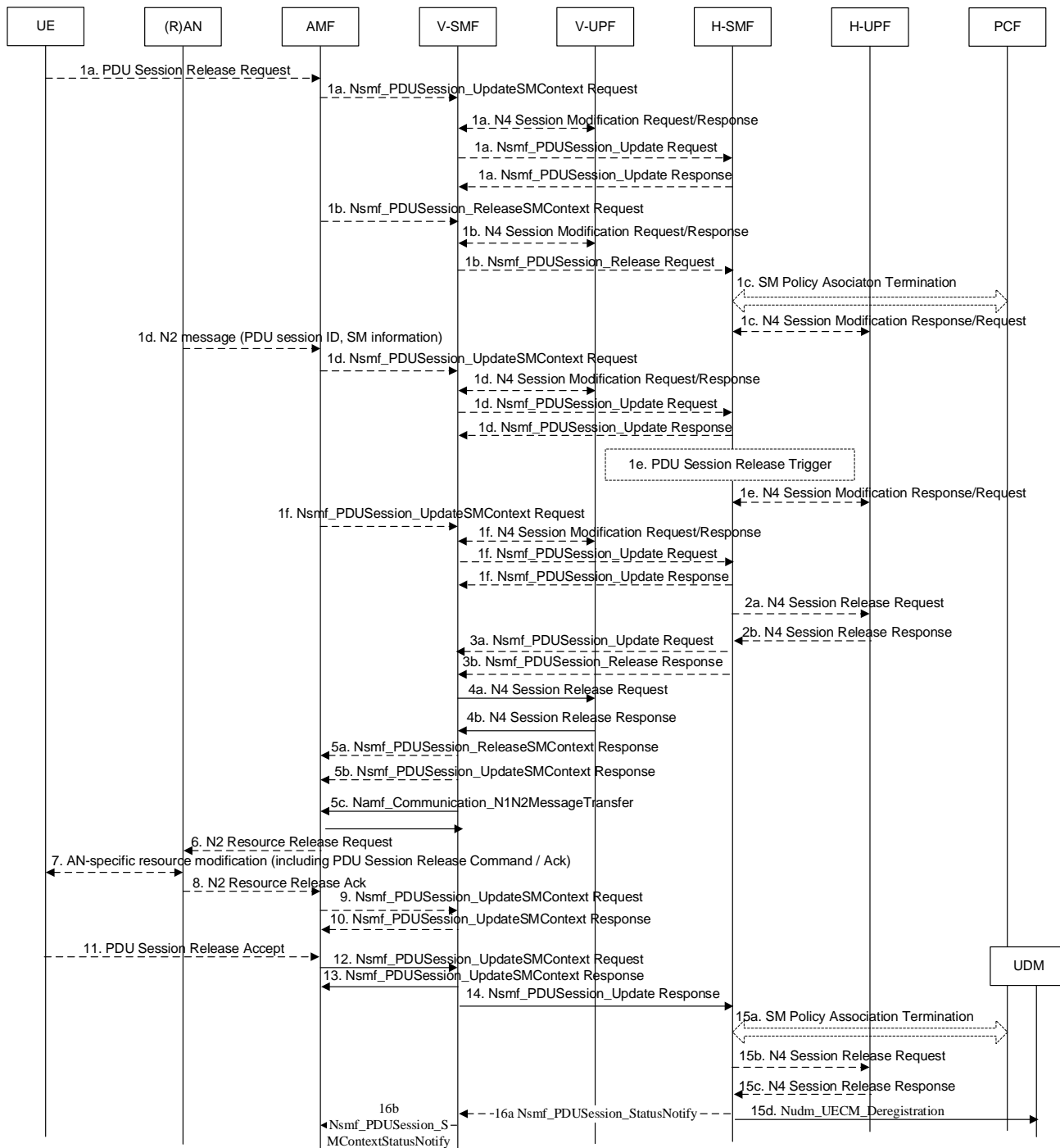
Figure 4.3.4.3-1: UE or network requested PDU Session Release for home-routed roaming
