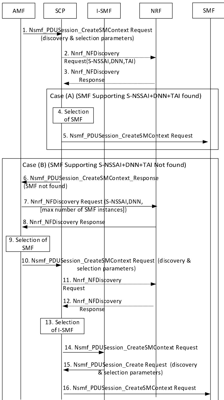
Figure E.2: Delegated Discovery of I-SMF
