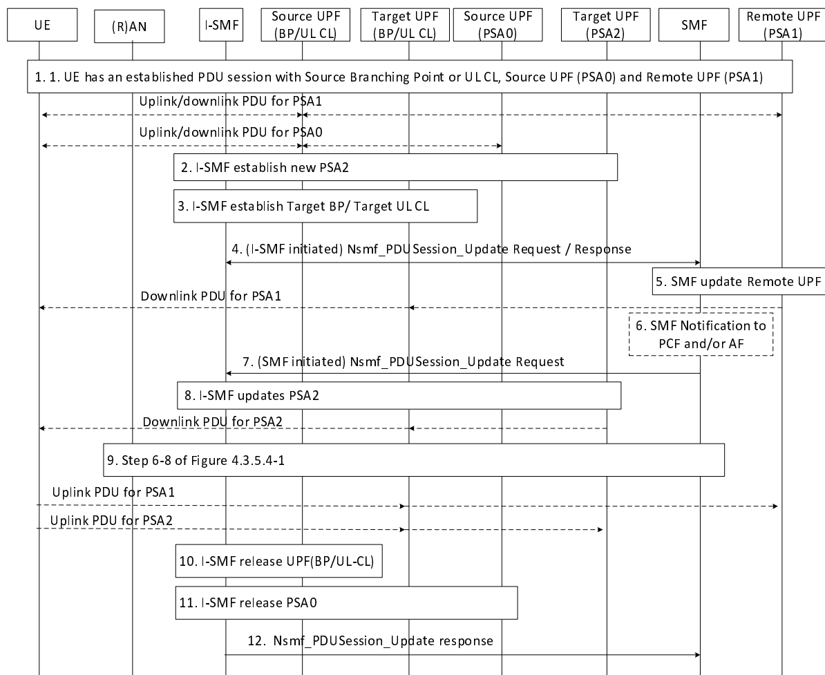
Figure 4.23.9.4-1: Simultaneous change of Branching Point or UL CL and additional PSA controlled by I-SMF
