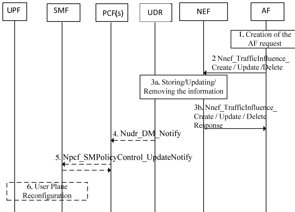
Figure 4.3.6.2-1: Processing AF requests to influence traffic routing for Sessions not identified by an UE address
