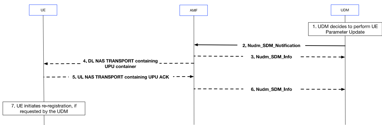
Figure 4.20.2-1: UE Parameters Update via UDM Control Plane Procedure
