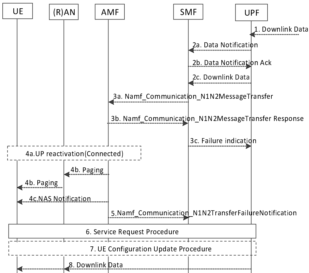
Figure 4.2.3.3-1: Network Triggered Service Request
