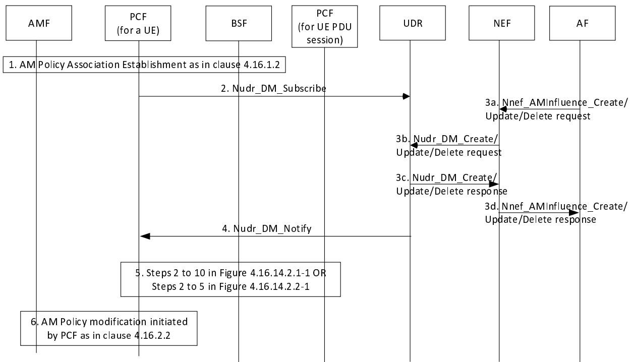
Figure 4.15.6.9.3-1: Handling an AF request to influence AM Policy
