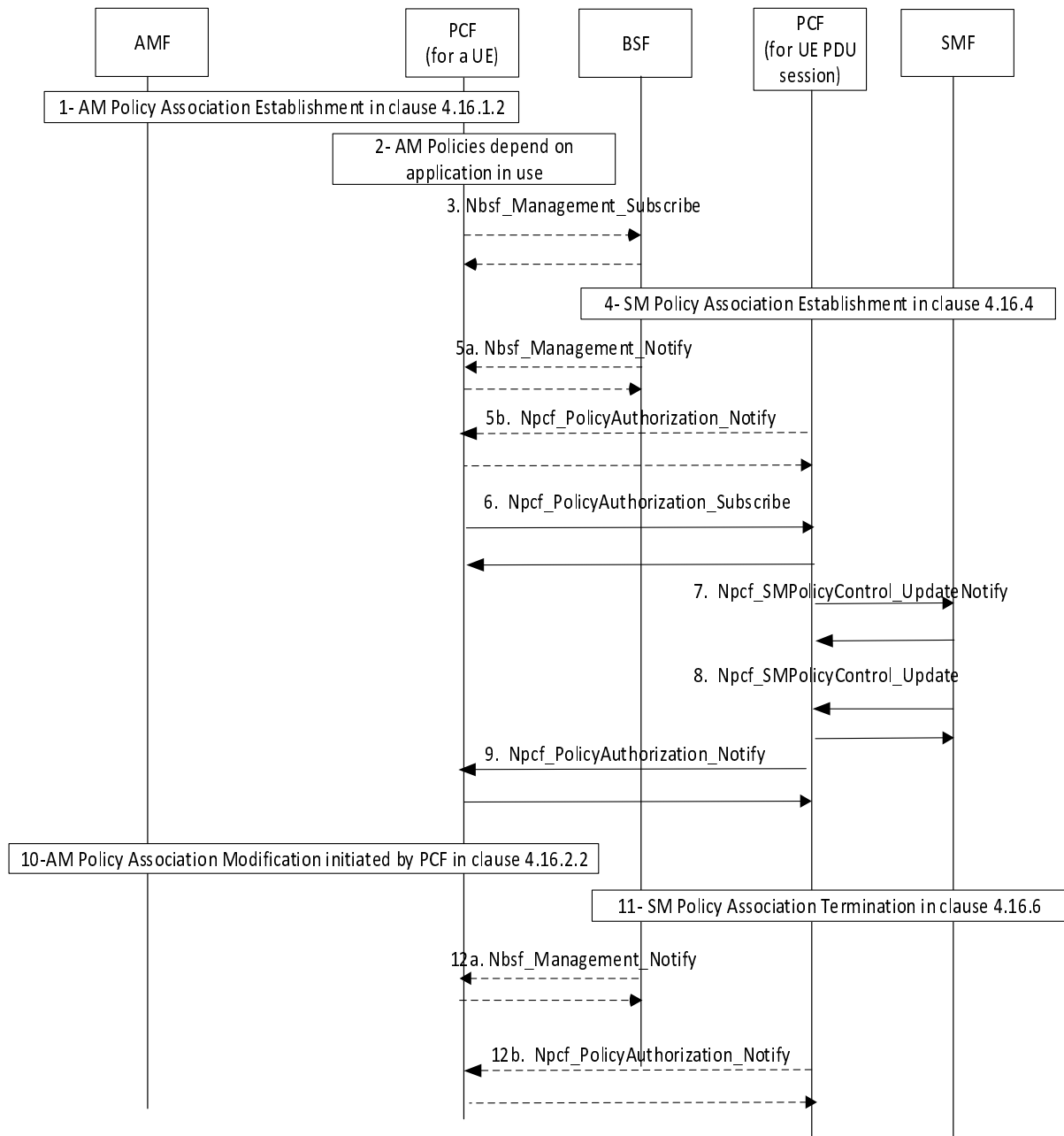
Figure 4.16.14.2.1-1: Management of AM Policies at start and stop of application traffic
