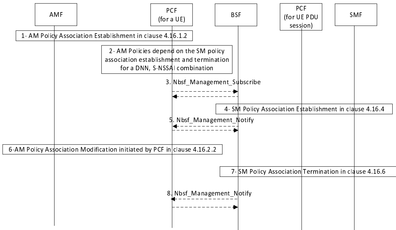
Figure 4.16.14.2.2-1: Management of AM Policies at SM policy association establishment and termination with the notification by the BSF
