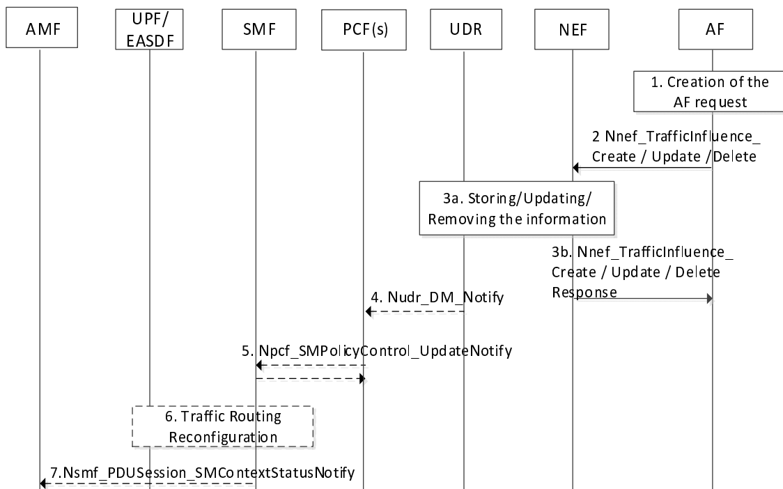
Figure 4.3.6.2-1: Processing AF requests to influence traffic routing for Sessions not identified by a UE address
