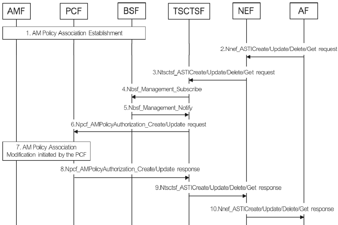
Figure 4.15.9.4-1: Management of 5G access stratum time information
