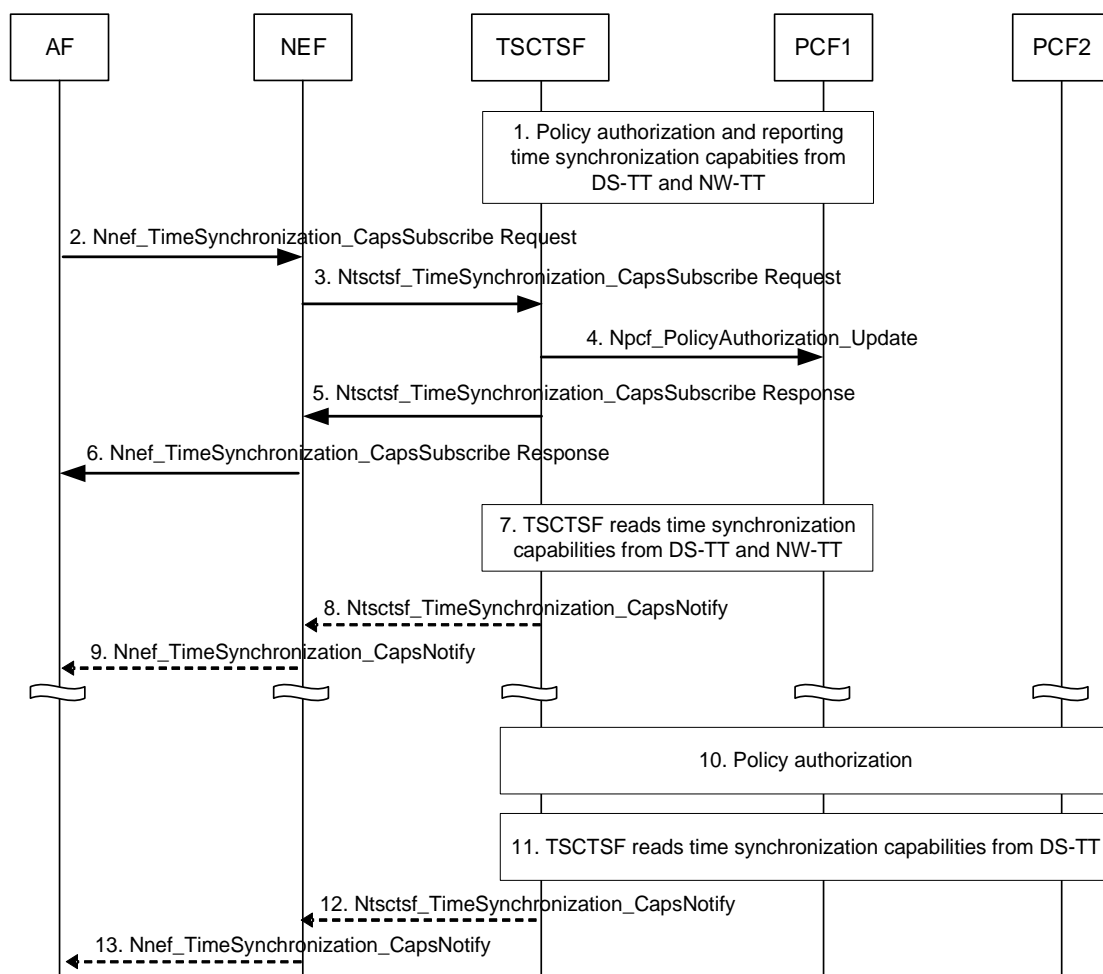
Figure 4.15.9.2-1: Procedure for exposing 5GS and/or UE availability and capabilities for Time Synchronization services
