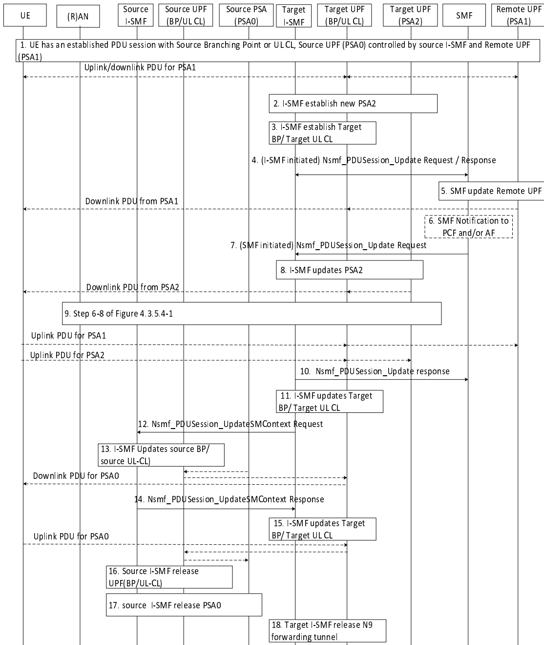
Figure 4.23.9.5-1: Simultaneous change of Branching Point or UL CL and additional PSA controlled by different I-SMFs
